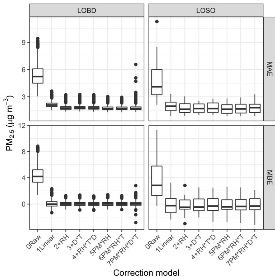
965 Figure 4. Performance statistics including mean bias error (MBE) and mean absolute error (MAE) are shown by correction method (0-7), where each point in the boxplot is the performance for either a 12-week period excluded from correction building (“LOBD”), or a single state excluded from correction building (“LOSO”).
