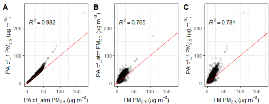
960 Figure 3. Comparison of the 24-hour raw PurpleAir (PA) cf_1 and cf_atm PM 2.5 outputs (A) and both outputs compared to the FEM or FRM PM 2.5 measurements (B and C) across all sites with the 1:1 line in red.
