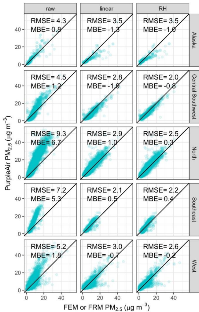
975 Figure 6. Scatterplot of the daily FEM or FRM \text{PM}_{2.5} data with the PurpleAir data by U.S. region (see Figure 2) prior to any correction, after applying a linear correction, and after applying the final correction including RH. Data were corrected using the models built for the full dataset.
