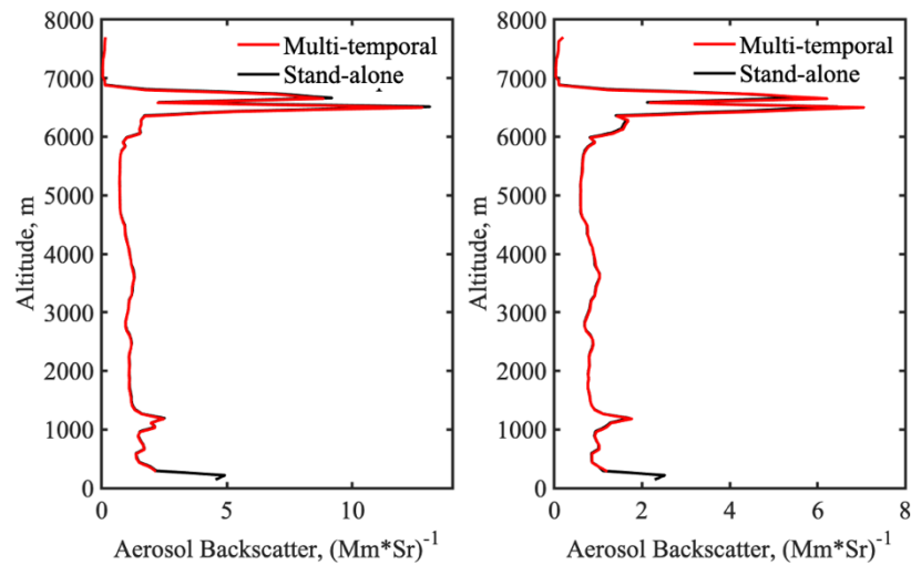
Figure 24: Aerosol backscatter profiles at 455nm (left) and 940 nm (right) estimated from COBALD profiles acquired on 5 August 2015 using a stand-alone (black) and multi-temporal (red) retrieval schemes.
