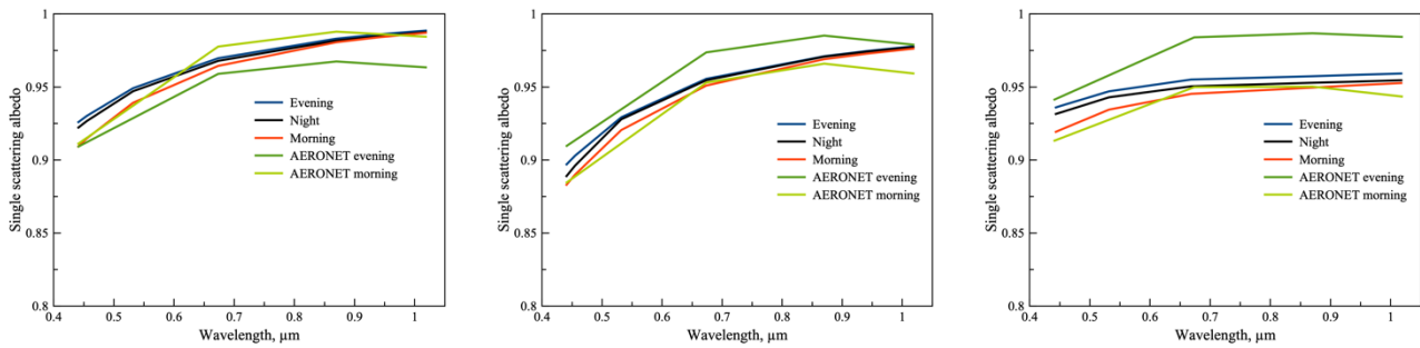
Figure 8: Aerosol single scattering albedo retrieved during COBALD sound flight on 5 of August 2015 (left), 11 of August 2015 (center) and 12 of August 2016 (right). Values retrieved before and after the radiosonde flight with use of combined sun photometer and MPL data are shown in blue and red, retrieved by AERONET — in dark and light green, respectively.
