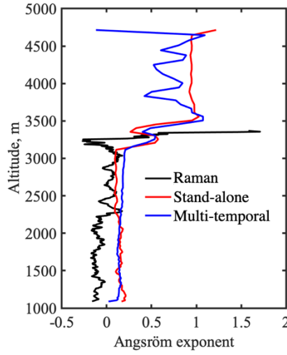
Figure 34: Vertical profile of Angström exponent at 355/532 nm retrieved from LILAS observations using stand-alone (red) and multi-temporal approaches (blue) performed on 16 of April 2015 in comparison with estimation from 355/532 inelastic backscatter measurements (black).
