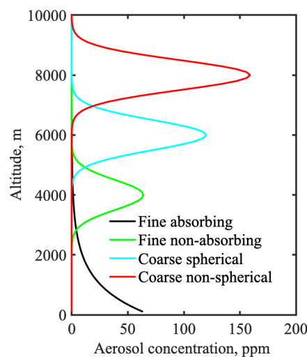
Figure 30: Aerosol vertical distribution used for the simulation in the LILAS sensitivity test.
