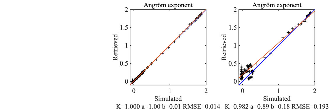
Figure 20: Comparison between simulated and retrieved Angström exponent profiles at 455/940 nm in noise free (left) and noisy (right) conditions.
