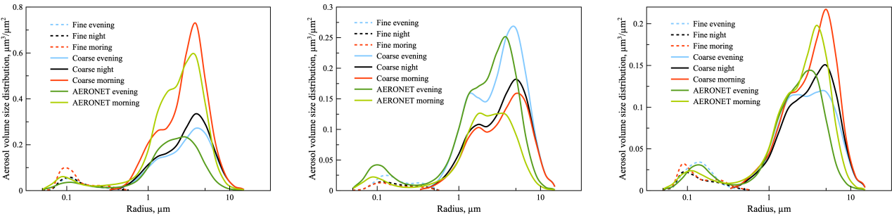
Figure 4: Aerosol volume size distributions for fine (dashed) and coarse (solid) aerosol components retrieved during COBALD sound flight on 5 of August 2015 (left), 11 of August 2015 (center) and 12 of August 2016 (right). Distributions retrieved before and after the radiosonde flight with use of combined sun photometer and MPL data are shown in blue and red, retrieved by AERONET — in dark and light green, respectively.
