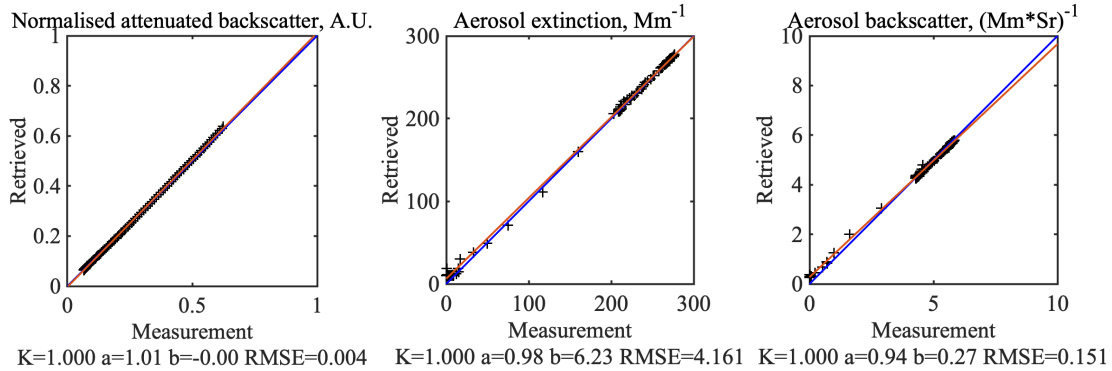
Figure 36: Achieved fits for attenuated inelastic backscatter at 387 (left) aerosol extinction at 532 nm (middle) and aerosol backscatter at 532 nm (right), data acquired on 16 of April 2015.
