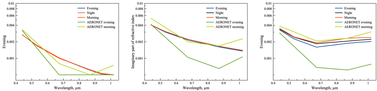
Figure 7: Imaginary parts of aerosol complex refractive indices retrieved during COBALD sound flight on 5 of August 2015 (left), 11 of August 2015 (center) and 12 of August 2016 (right). Values retrieved before and after the radiosonde flight with use of combined sun photometer and MPL data are shown in blue and red, retrieved by AERONET — in dark and light green, respectively.
