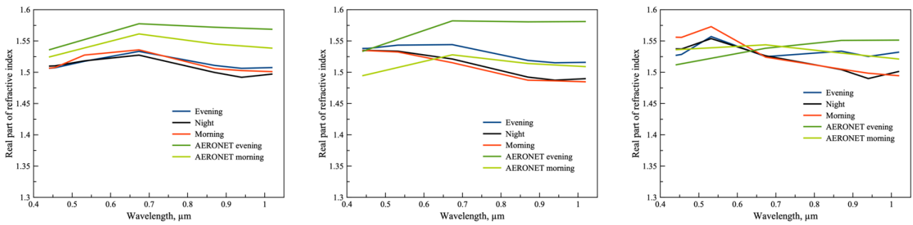
Figure 6: Real parts of aerosol complex refractive indices retrieved during COBALD sound flight on 5 of August 2015 (left), 11 of August 2015 (center) and 12 of August 2016 (right). Values retrieved before and after the radiosonde flight with use of combined sun photometer and MPL data are shown in blue and red, retrieved by AERONET — in dark and light green, respectively.
