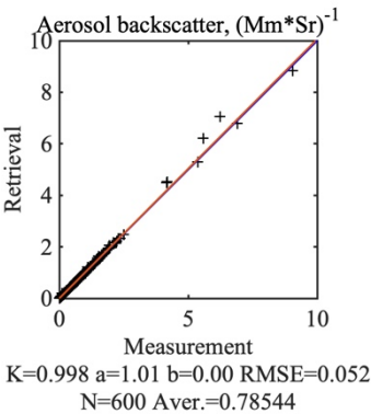
Figure 11: Achieved backscatter fits for the multi-temporal retrievals performed at 5, 11 of August 2015 and 12 of August 2016.
