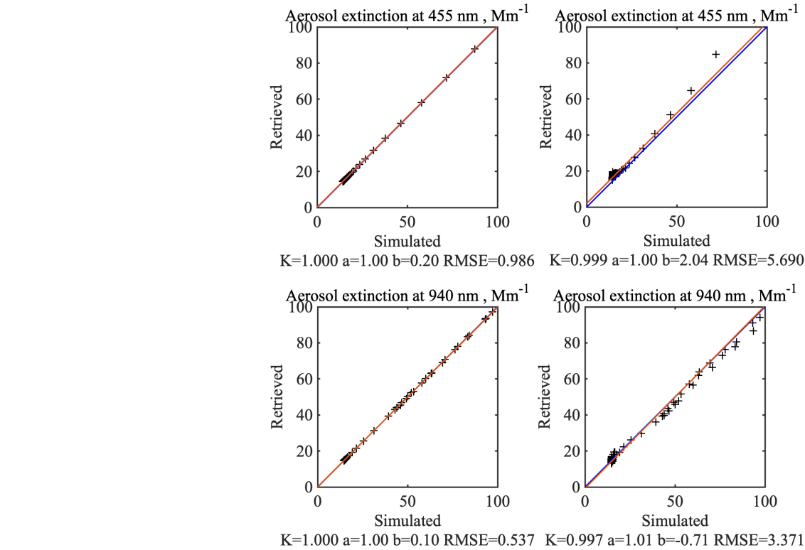
Figure 19: Comparison between simulated and retrieved aerosol extinction profiles at 455 (top) and 940 (bottom) nm in noise free (left) and noisy (right) conditions.
