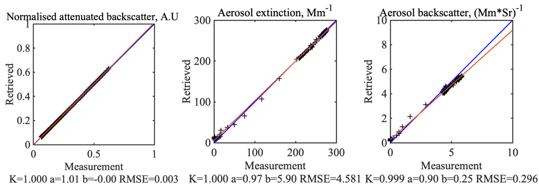
Figure 17: Achieved attenuated normalized inelastic backscatter (left), aerosol extinction (middle) and aerosol backscatter (right) fits for the synergy retrievals performed on 15–16 of April 2015.
