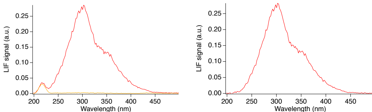
545 Figure 4. Fluorescence spectrum observed from SO 2 (red) in addition to Rayleigh scattering and background (orange) (left) and the absolute SO 2 fluorescence after subtraction of the background (right).
