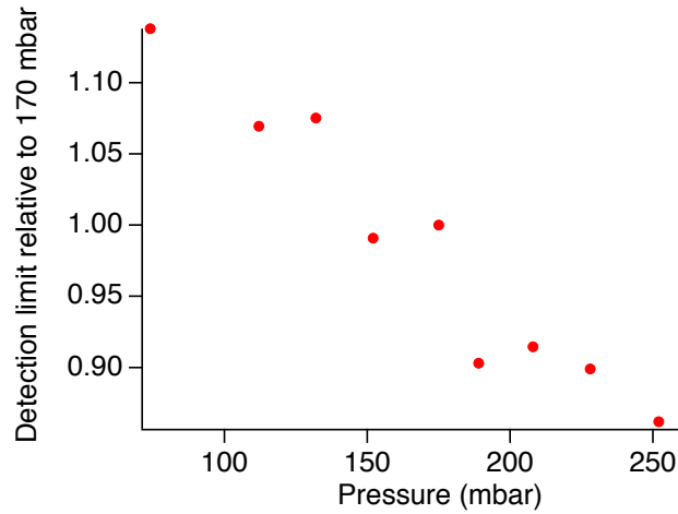
565 Figure 8. Measured LIF SO 2 detection limit over a pressure range of 74-277 mbar.
