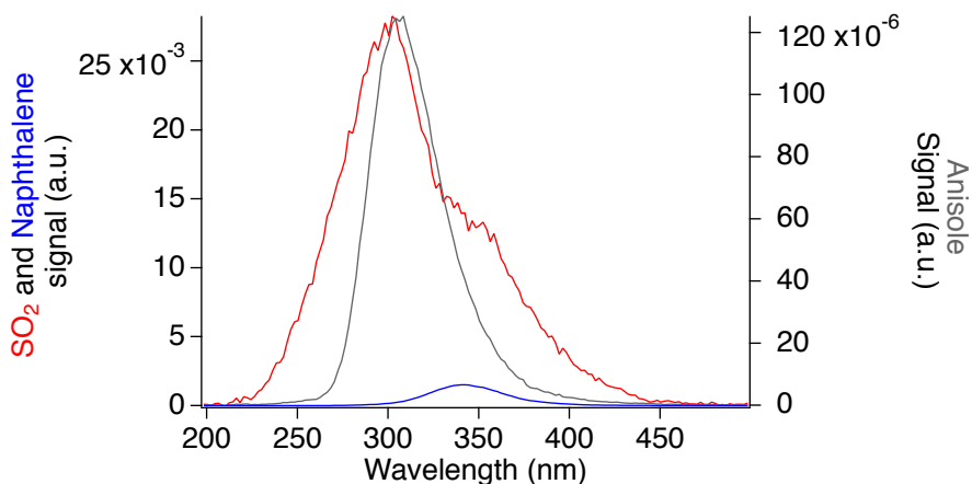
Figure 5. Fluorescence spectra of SO 2 (red), naphthalene (blue), and anisole (grey) normalized by the calculated concentrations.
