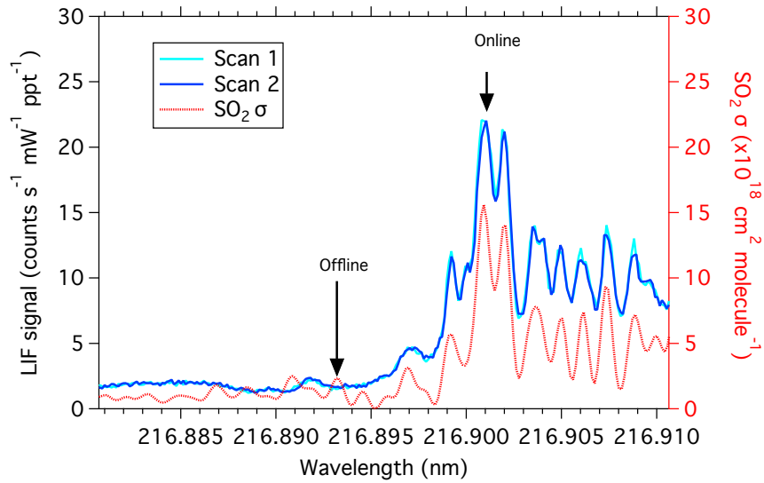
530 Figure 1. SO 2 absorption cross-section (red, right axis) in comparison to laser scans by the LIF SO 2 instrument (blue and cyan, left axis). The online wavelength is identified as the largest absorption cross-section peak.
