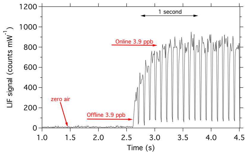
535 Figure 2. SO 2 measurements performed at 10 Hz showing a large distinction between online and offline signals. Background measurements with zero air show the signal to be negligible in the absence of SO 2 .
