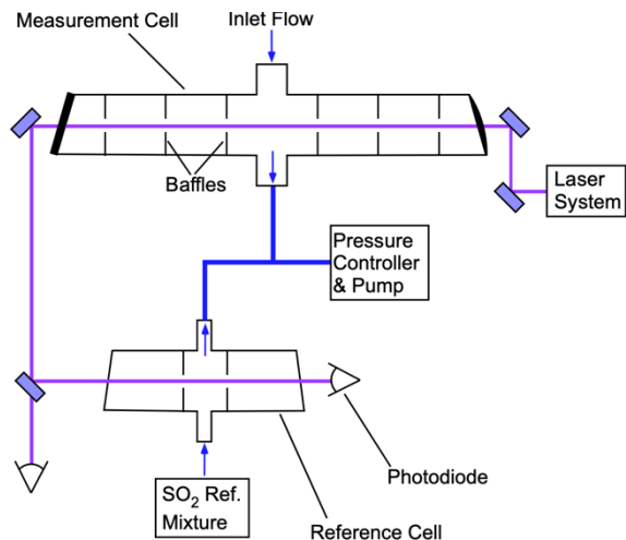
540 Figure 3. LIF SO 2 detection optical bench. PMTs are located above the plane of this schematic and oriented to collect fluorescence from the center of each cell.
