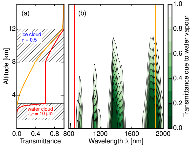
Figure 4. (a) Atmospheric transmittance of a water cloud and overlying ice cloud layer at 870\text{nm} (red line) and 1.9\text{ }\mu\text{m} (orange line) (b) The spectral transmittance of atmospheric water vapour acting as a vertical weighting function.
