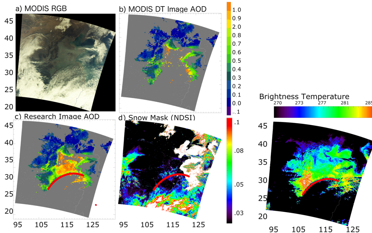
Example figure, A pollution event over eastern China on Terra MODIS sensor with granule id of 2013348.0310. a) MODIS Terra RGB image, b) MODIS Dark Target (DT) AOD at .055 \mu\text{m} for all available retrievals (QA = 0 to 3), c) Research AOD at 0.55 \mu\text{m} , for all available retrievals, d) Snow mask, e) 11 \mu\text{m} Brightness Temperature map. The red line shows the cloud edge.
