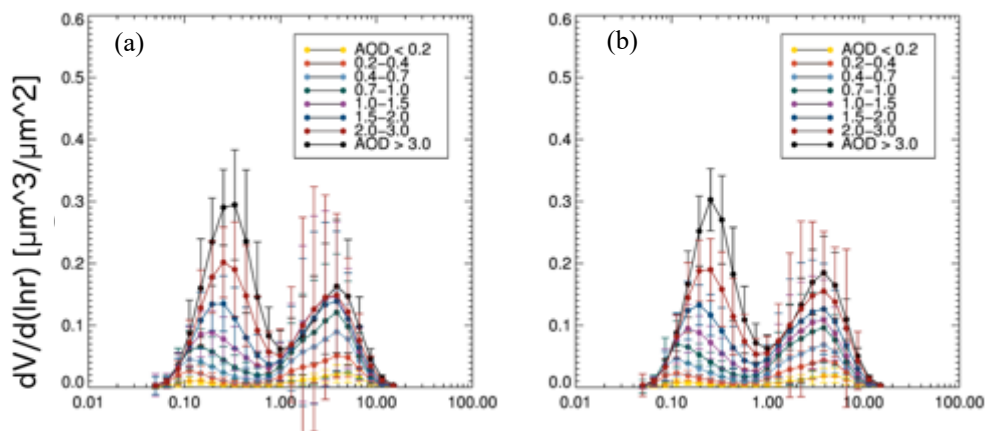
Figure 5: Size distribution as a function of AERONET AOD at 0.675 \mu\text{m} , generated from the AERONET inversion products at cluster 1 illustrated in Figure 3 using all available data records, a) is from April to September, b) is from October to March. The error bars represent the standard deviation within each size bin.
