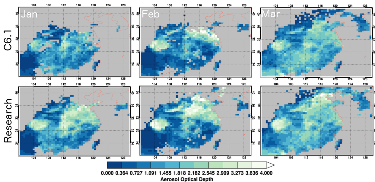
850 Figure 13 Spatial distribution of averaged AOD from the operational product (upper row) and the research product (lower row) at 0.5° resolution over the study domain from January to March 2013.
