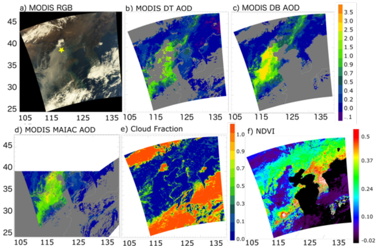
785 Figure 1 A case study of a pollution event over eastern China on 9 October, 2013. a) MODIS Aqua RGB image, b) MODIS Dark Target (DT) AOD at 0.55\ \mu\text{m} for all available retrievals (QA = 0 to 3), c) MODIS Deep Blue (DB) AOD at 0.55\ \mu\text{m} , for all available DB retrievals (QA = 0 to 3) d) MODIS MAIAC AOD e) MODIS DT Cloud Fraction , a diagnostic of the MODIS aerosol product, f) Normalized Difference vegetation index, used as the inland water mask by the DT algorithm . The yellow star represents the AERONET site Xianghe.
