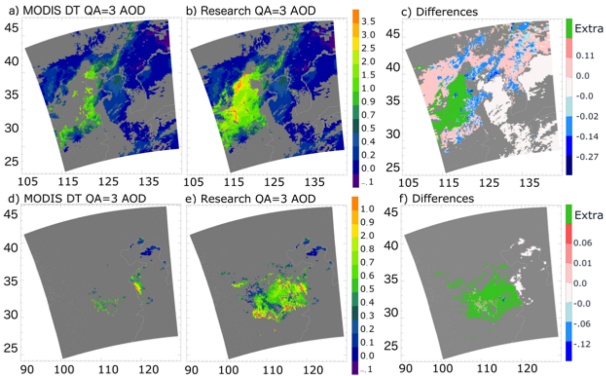
Figure 8 a) to c) AOD images for the case study over Eastern China on 9 October, 2013: a) operational DT AOD at 0.55 \mu\text{m} with QA = 3, b) Research AOD at 0.55 \mu\text{m} with QA = 3 using altered thresholds on the NDVI test, snow test, and a new regional aerosol model with new aerosol scale height. c) The differences between the research AOD (panel b) and the DT AOD (panel a). d) to f) are for a case study of moderate pollution over Eastern China on 13 December 2018. The increased research AOD data coverage is shown in green.
