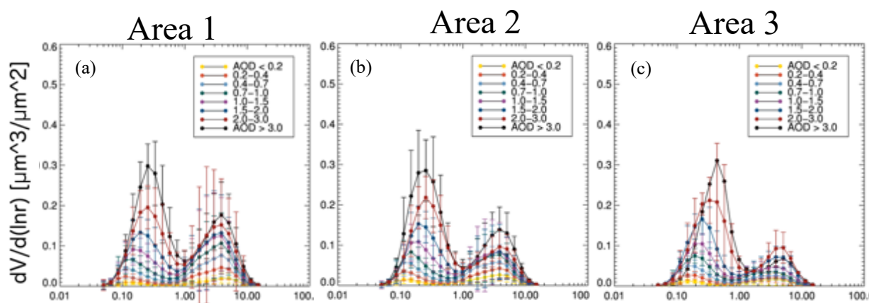
Figure 4: Size distribution as a function of AERONET AOD at 0.675 \mu m , generated from the AERONET inversion products at three clusters illustrated in Figure 3 using all available data records. Other than the last AOD bin, which is AOD > 3 , the number of retrievals within each AOD bin are between hundreds to thousands. There are 263, 15, and 1 data points in the highest AOD bin for cluster 1, 2, and 3, respectively. The error bars represent the standard deviation within each size bin
