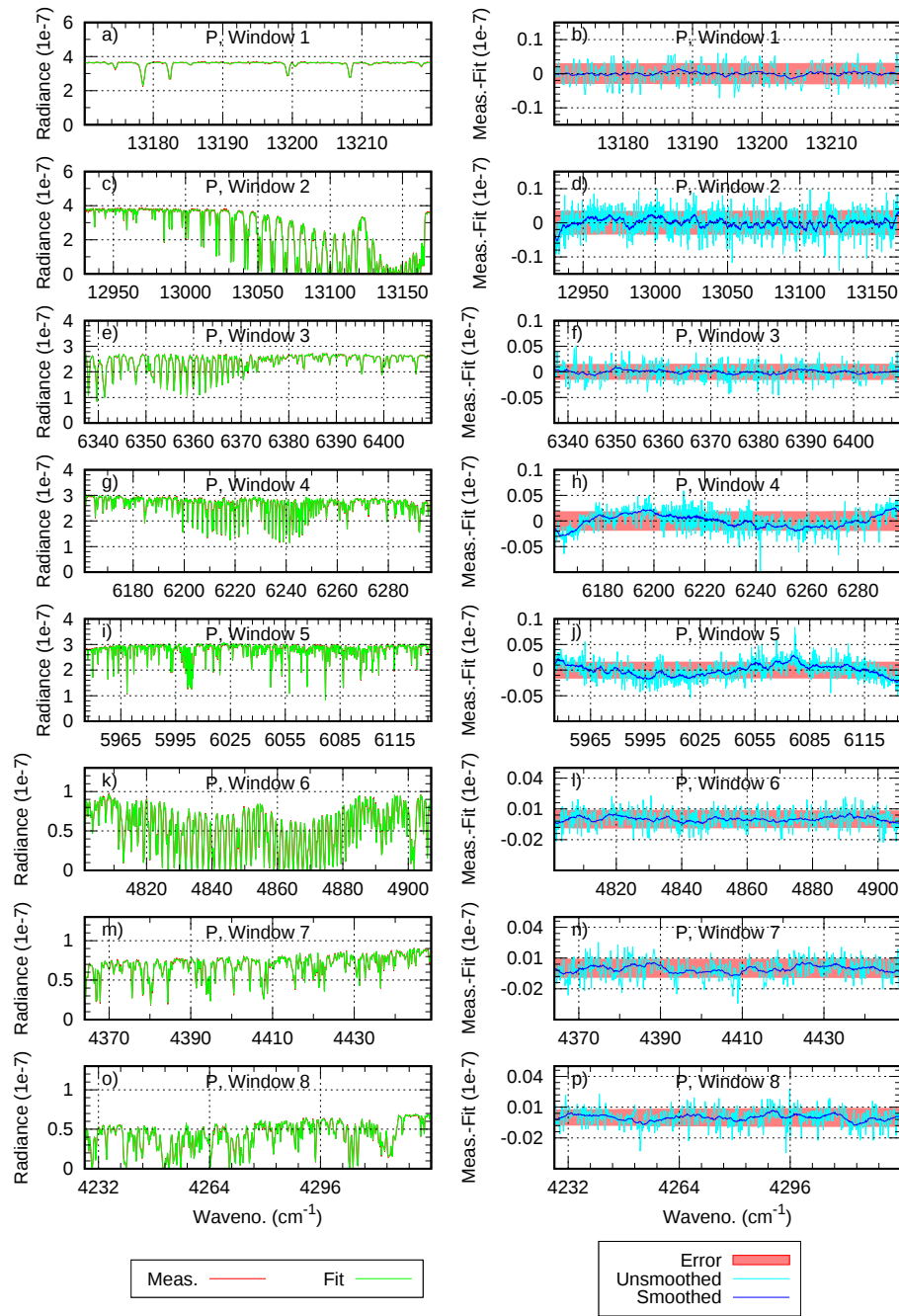
Figure 9. Same as Fig. 8, but for GOSAT-2.
