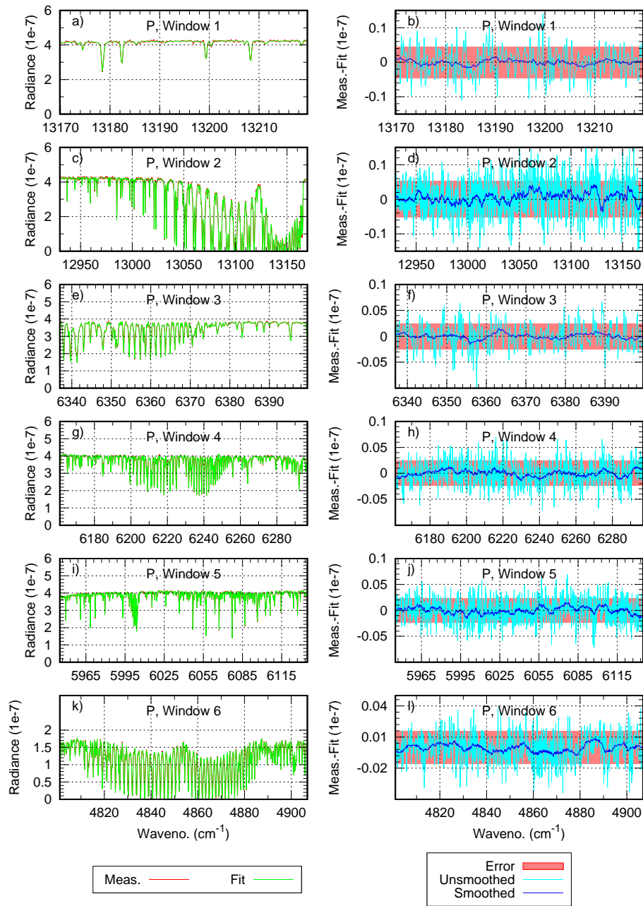
Figure 8. Example for a single GOSAT measurement (S-P polarisation): Left: Measured (red) and retrieved (green) spectra in the different fit windows; because of the good agreement the red curve is essentially barely visible below the green curve. Right: Corresponding residuals (measurement - fit). Light Blue: Unsmoothed. Blue: Smoothed with a boxcar of width 21 spectral pixels ( = 4.2 \text{ cm}^{-1} ). Red: Estimated noise error range. Radiance unit is \text{W}/\text{cm}^2/\text{cm}^{-1}/\text{sr} .
