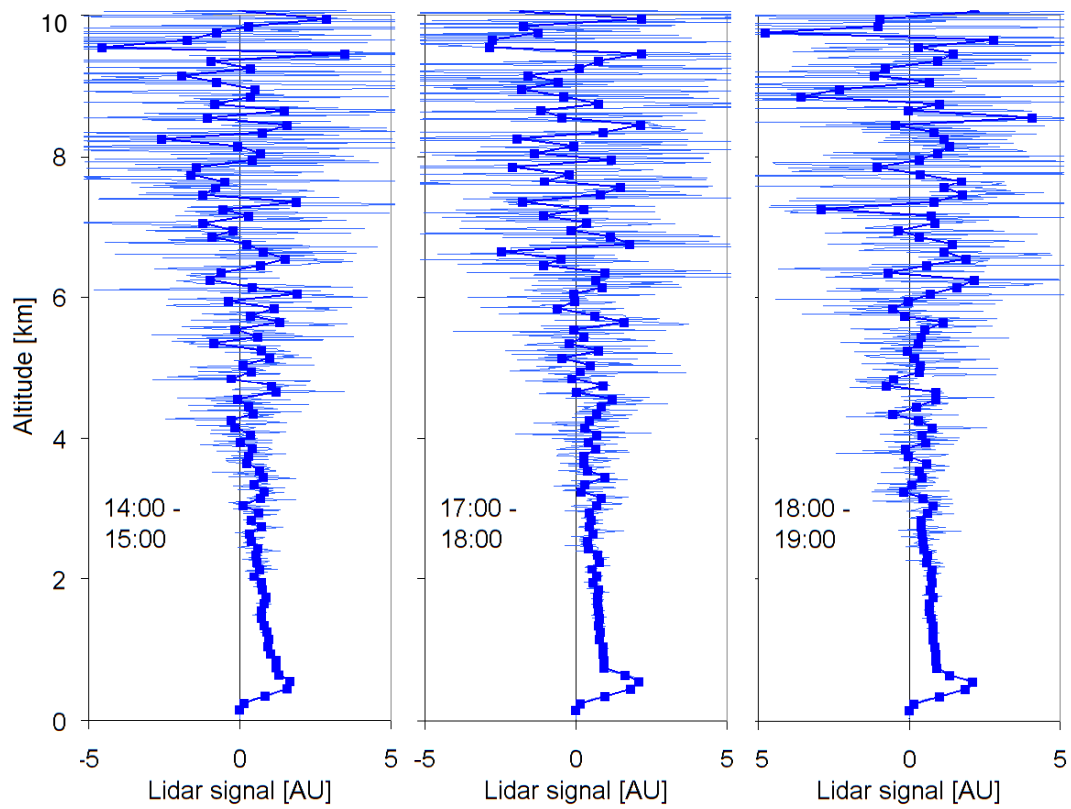
635 Fig. 4: Hourly averaged and range corrected ceilometer backscatter profiles for 3 periods on 2 May 2019 without cloud contamination. The thin lines represent the raw data. The dotted lines represent the smoothed profiles (averages over 100 m). The scatter of the range corrected backscatter profiles increases, because the received raw signal scales with the inverse of the square of the distance.
