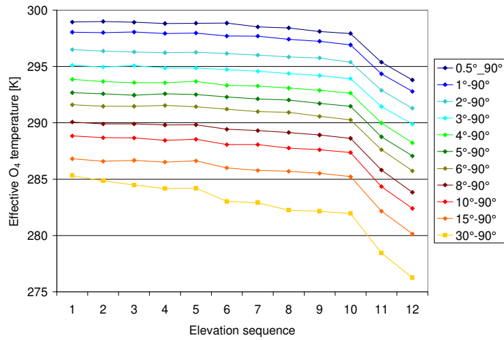
825 Fig. A9A10: Effective temperatures calculated for the individual measurements according to equation 2.
