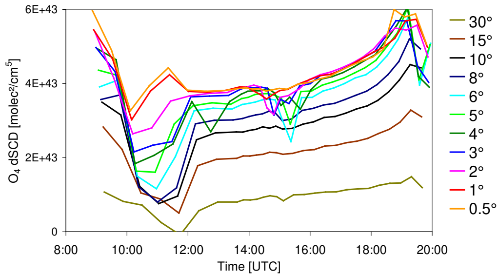
780 Fig. A3A4: Time series of the retrieved O 4 dSCD on 2 May 2019 for the different elevation angles. During the afternoon, for most of the time smooth variations are found. However, for some times and elevation angles systematic deviations of the O 4 dSCDs occur, which are caused by scattered clouds.
