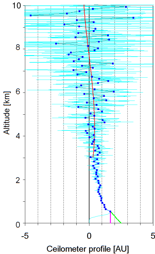
815 Fig. A8A9: The light blue data show the original backscatter profile averaged between 14:00 and 15:00. The blue dots show the smoothed (with a 100m kernel) profile, which are used between 500 m and 3 km. Below 500m either constant or linearly extrapolated data (see text) are used. Between 3 km and 10 km a third order polynomial is fitted to the raw data. The polynomial values are used between 3 km and the altitude at which they become negative. Above, the values are set to zero. 820
