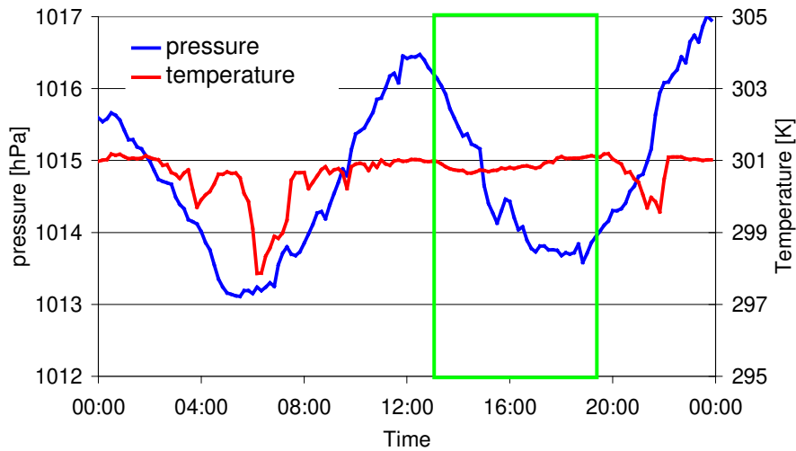
790 Fig. A4A5: Diurnal variation of the surface pressure and temperature from in situ measurements on the ship. The green box indicates the period of the MAX-DOAS measurements used in this study. The corresponding values from the ECMWF model simulations are 1012.8 hPa and 299.8 K, respectively.
