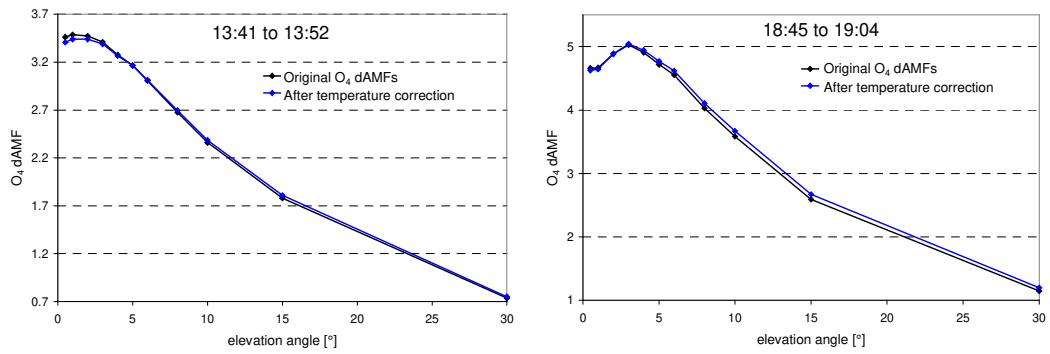
830 Fig. A10A11: Effect of the temperature correction for two selected elevation sequences.
