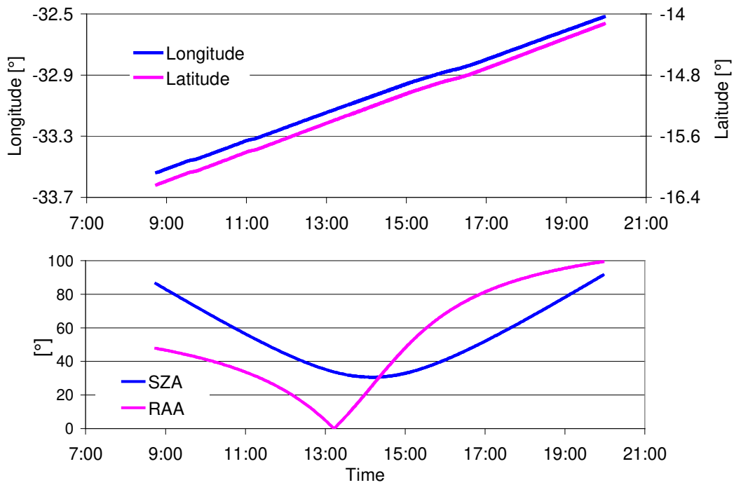
795 Fig. A5A6: Top: Variation of the latitude and longitude of the ship position during 2 May 2019. Bottom: Corresponding variation of the SZA and relative azimuth angle (RAA).
