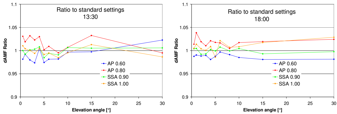
810 Fig. A7A8: Effect of different phase functions and single scattering albedos on the O_4 dSCDs. Shown are the ratios for simulations with variations of asymmetry parameter (AP) and single scattering albedo (SSA) versus simulations using the standard settings (AP= 0.68, SSA: 0.95). The results are for SZA of 33.6^\circ and RAA of 0.7^\circ (left, around 13:30) and SZA of 64.5^\circ and RAA of 87.7^\circ (right, around 18:00) on 2 May 2019). The results for other SZA/RAA combinations during the afternoon of 2 May 2019 are similar.
