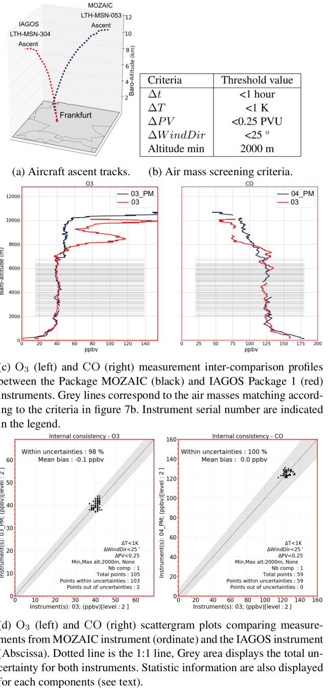
Figure 7. O 3 and CO profile inter-comparisons on 2012/12/17 between MOZAIC Luthansa msn-053 and IAGOS Luthansa msn-304. Both aircraft ascent from Frankfurt airport within a 13 minutes time interval. The MOZAIC aircraft is equipped with the instrument unit serial number 03 PM for O 3 and 04 PM for CO. The Package 1 mounted on the IAGOS aircraft is serial number 03.
