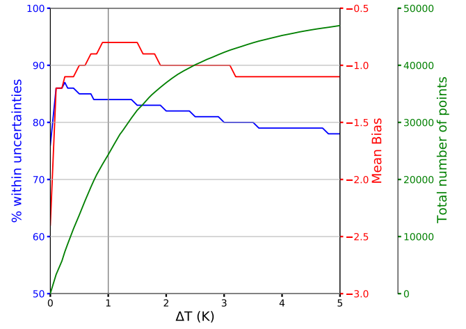
Figure 9. Percentage of points within the uncertainty and mean bias as function of the potential temperature difference measured by the co-located aircraft found for CO instrument 04 PM and for the flight period number 13 on Lufthansa A340msn53. The total number of comparable points according the air temperature difference is also shown. The maximum time difference between the landings or the take offs is 1 hour.
