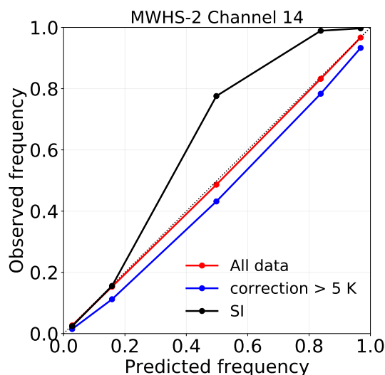
Figure 6. Calibration of the prediction intervals derived from QRNN-single (89+150 GHz) for MWHS-2 channel 14, and prediction intervals derived from Gaussian error model for ECMWF NWP system (SI). For the former, the calibration for both the entire predicted dataset and the subset with correction greater than 5 K are shown.
