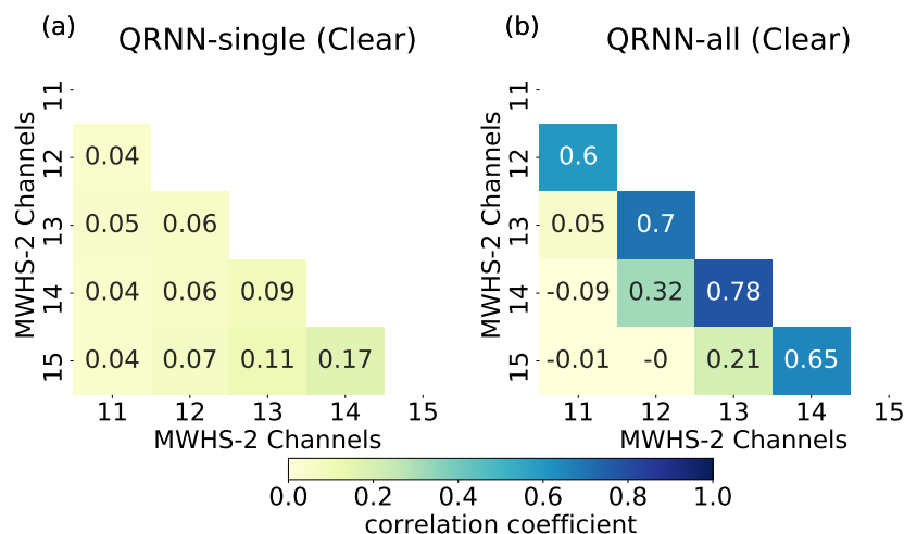
Figure 4. The triangular error correlation matrix obtained from (a) QRNN-single and (b) QRNN-all for MWHS-2. The label “Clear” represents cases with cloud impact less than 2 K.
