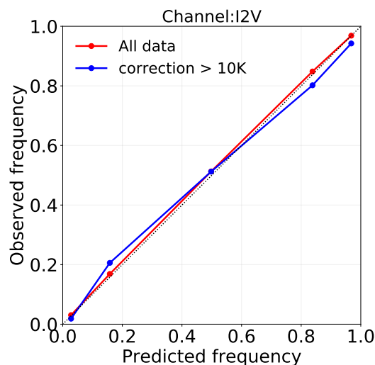
Figure 10. Same as Fig. 6, but from QRNN-single for ICI channel I2V.
