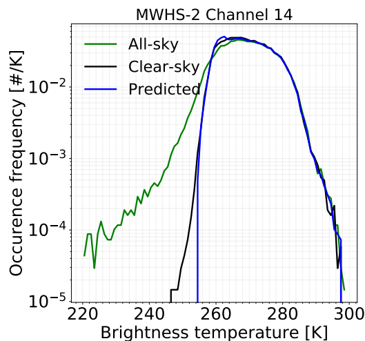
Figure 2. The distribution of point estimates (“Predicted”) obtained from QRNN-single 89+150 GHz for MWHS-2 channel 14. The corresponding distributions for all-sky and clear-sky simulations are also shown.
