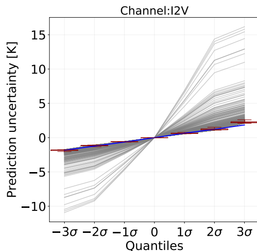
Figure 9. Same as Fig. 5, but from QRNN-single for ICI channel I2V. The blue line represents a Gaussian distribution with a standard deviation of 0.65 K.
