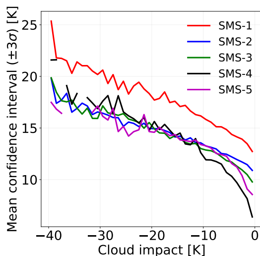
Figure 12. The average confidence intervals ( \pm 3\sigma ) plotted against the magnitude of cloud impact for all SMS channels.
