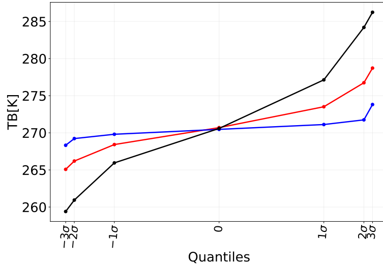
Figure 1. Examples showing the predicted quantiles of the conditional distribution of y_{\text{NFCS}}
