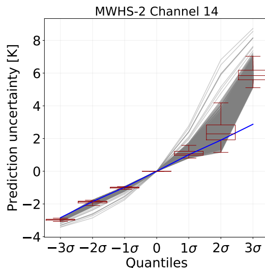
Figure 5. Examples of prediction uncertainties obtained from QRNN-single (89+150 GHz) for MWHS-2 channel 14. 1500 randomly selected cases are shown. The quantiles have been plotted at equidistant points. The blue line represents a Gaussian distribution with a standard deviation of 1.0 K. For each quantile, the sample variation is also shown as box plot.
