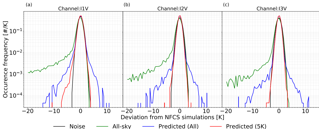
Figure 8. Same as Fig. 3, but from QRNN-single experiment for ICI channels (a) I1V, (b) I2V and (c) I3V.
