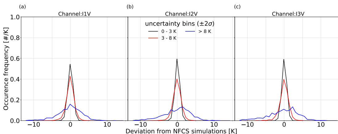
Figure 13. Distribution of errors binned according to their uncertainty. Results are from QRNN-single for channels I1V, I2V and I3V.
