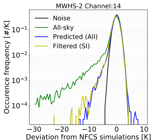
Figure 3. The error distribution for deviations of point estimates from NFCS simulations. The results are from QRNN-single experiment 89+150 GHz and MWHS-2 channel 14. Noise is also plotted for reference. The label “All-sky” represents the all-sky simulations, “Predicted (All)” denotes the predicted point estimates. The error distribution achieved with scattering index (SI) filtering is also shown (Filtered (SI)).
