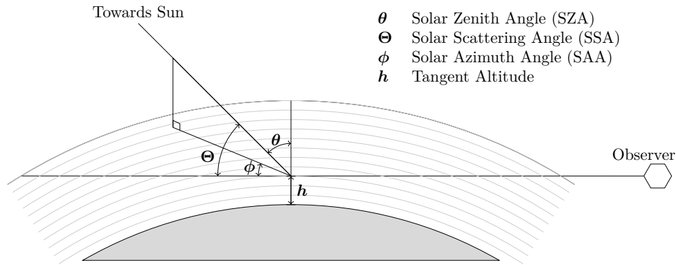
Figure 1. The limb viewing geometry and definitions of solar zenith angle, solar azimuth angle, solar scattering angle, and tangent altitude. The tangent altitude and solar zenith angles are defined relative to the un-refracted tangent point such that a solar scattering angle of 0^\circ is perfect forward scatter, and a solar zenith angle of 0^\circ is the sun directly overhead. Figure adapted from Zawada et al. (2015).
