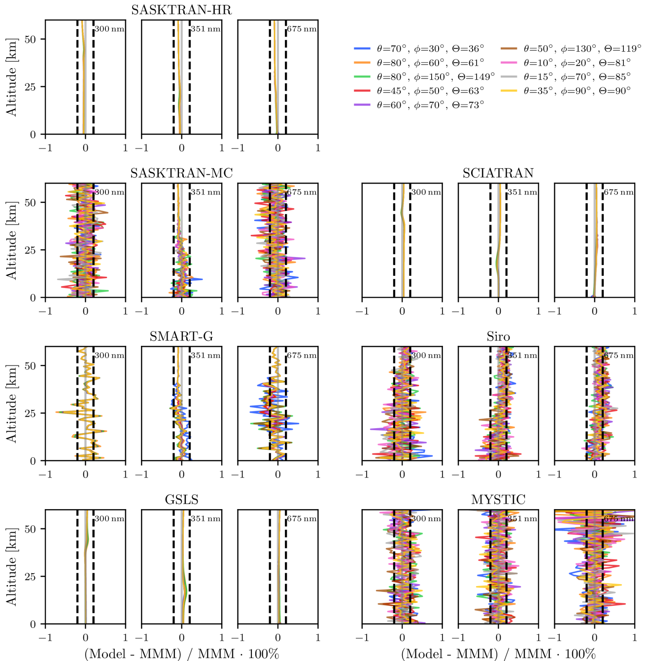
Figure 3. Percent differences in single scatter I relative to the MMM (GSLs, SASKTRAN-HR, and SCIATRAN) for each RTM at a variety of wavelengths and solar conditions. The atmospheric optical properties include Rayleigh scattering, ozone absorption, and stratospheric aerosol Mie scattering. Refraction is disabled. Dashed vertical lines indicate \pm 0.2\%
