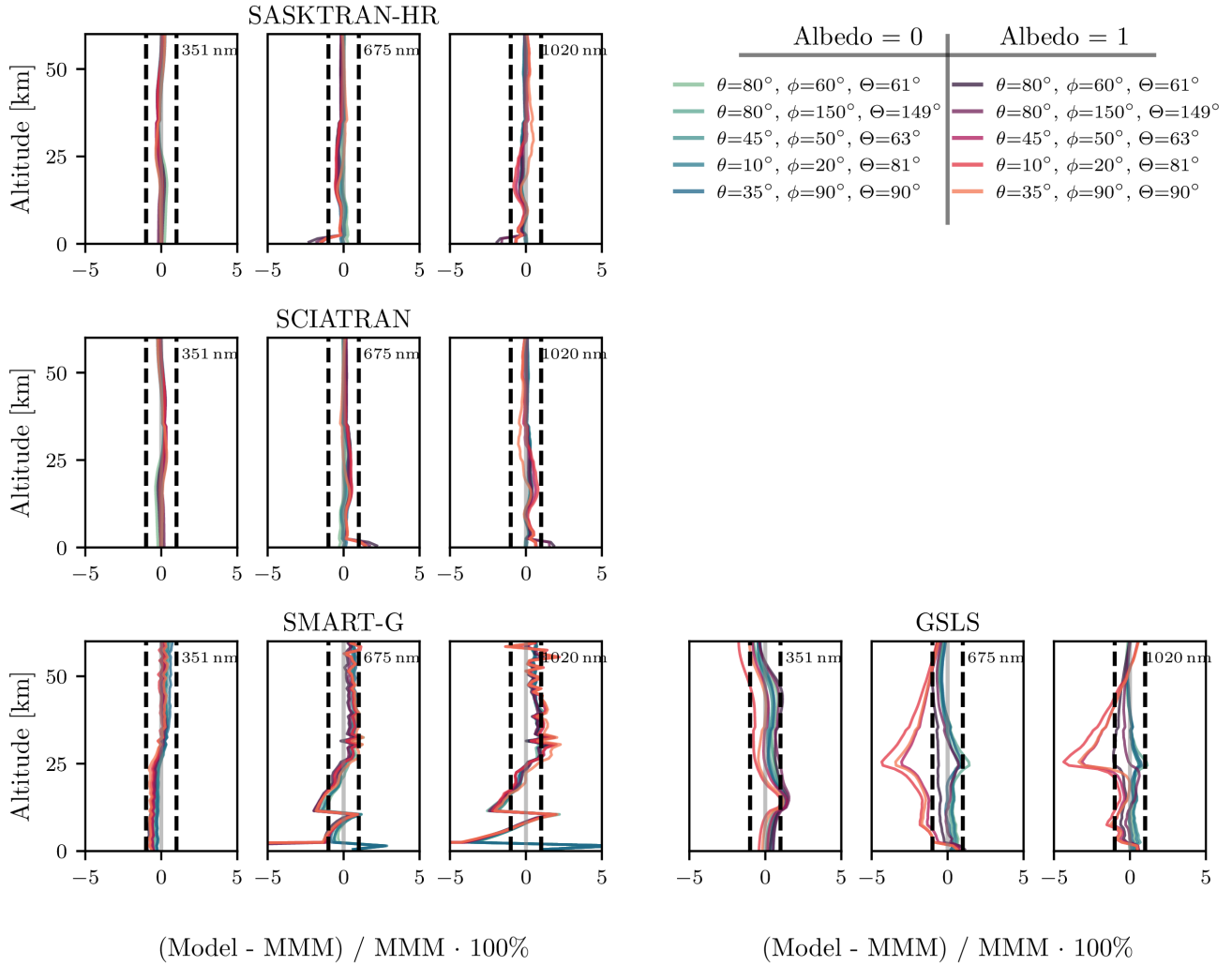
Figure 8. Same as Fig. 4 but with refraction enabled. The MMM is composed of SASKTRAN and SCIATRAN. Dashed vertical lines indicate \pm 1\% levels.
