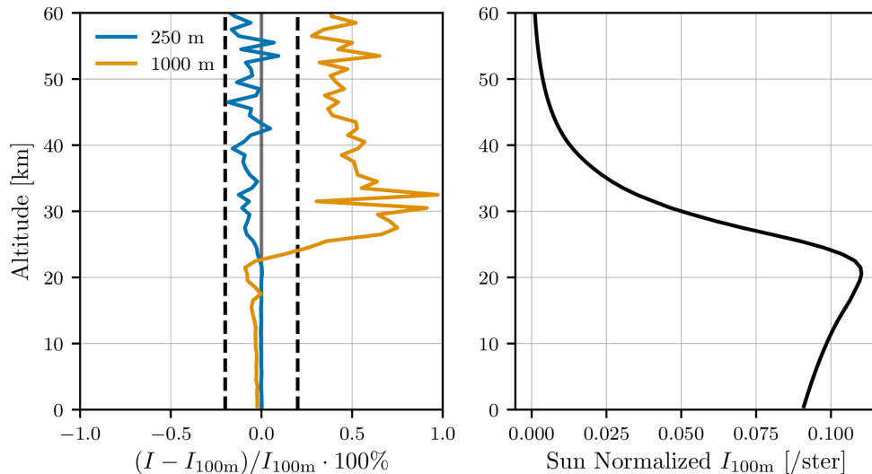
Figure 2. (Left Panel) Percent difference in single scattered radiance at 351 nm when MYSTIC is using 1000 m or 250 m homogeneous shells compared to 100 m homogeneous shells. (Right Panel) The sun-normalized radiance computed using 100 m shells. The atmosphere contains Rayleigh scattering, ozone absorption, and stratospheric aerosol Mie scattering with a SZA of 70^\circ and a SAA of 30^\circ . Refraction is disabled. MYSTIC was configured to use 100 million photons. Dashed vertical lines indicate \pm 0.2\% levels.
