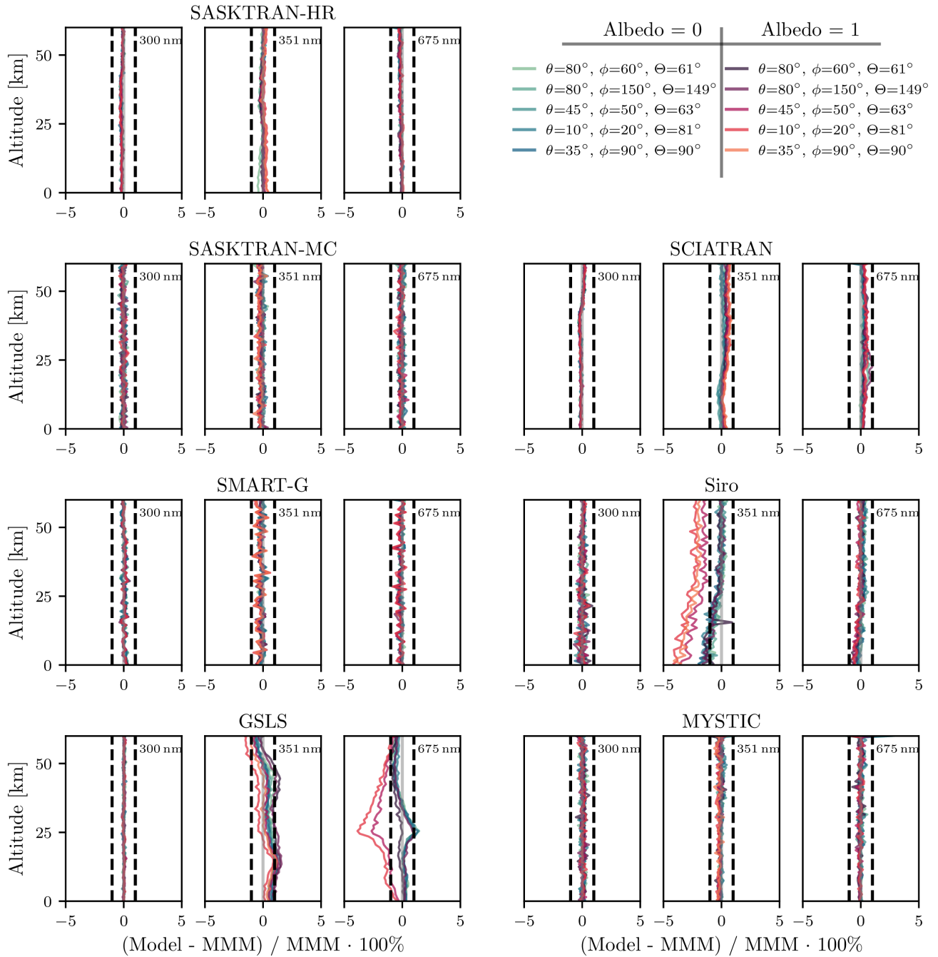
Figure 4. Percent differences in I , with multiple scattering enabled, relative to the MMM (MYSTIC, SASKTRAN-HR, SASKTRAN-MC, SCIATRAN, and SMART-G) for each RTM at a variety of wavelengths and solar conditions. The atmospheric optical properties include Rayleigh scattering, ozone absorption, and stratospheric aerosol Mie scattering. Refraction is disabled. Dashed vertical lines indicate \pm 1\% levels.
