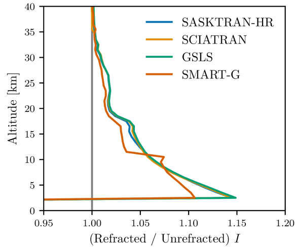
Figure 9. Ratio of refracted to unrefracted I with multiple scattering enabled, Rayleigh scattering + ozone absorption + stratospheric aerosol scattering, \text{SZA}=70^\circ , \text{SAA}=30^\circ , and a Lambertian surface reflectance of 0 at 1020 nm for every model that supports refraction.
