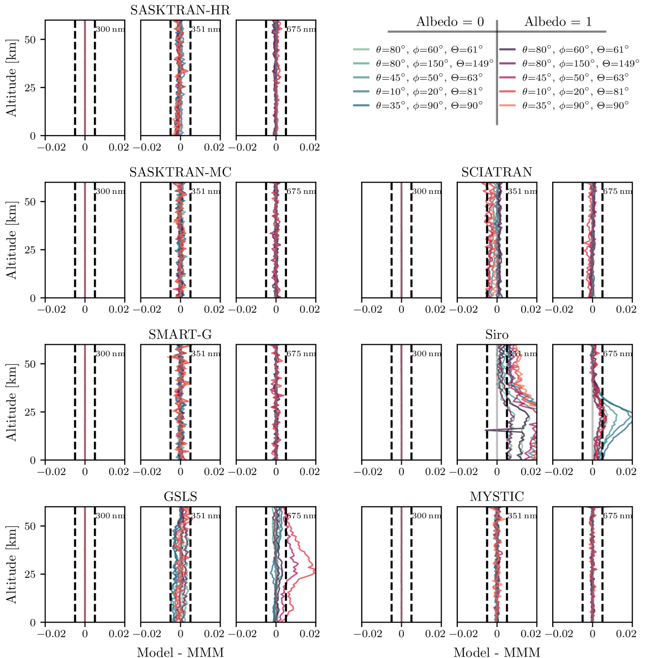
Figure 6. Absolute differences in DOLP relative to the MMM (MYSTIC, SASKTRAN-MC, and SMART-G) for each RTM at a variety of wavelengths and solar conditions. The atmospheric optical properties include Rayleigh scattering, ozone absorption, and stratospheric aerosol Mie scattering. Refraction is disabled. Dashed vertical lines indicate \pm 0.005 levels.
