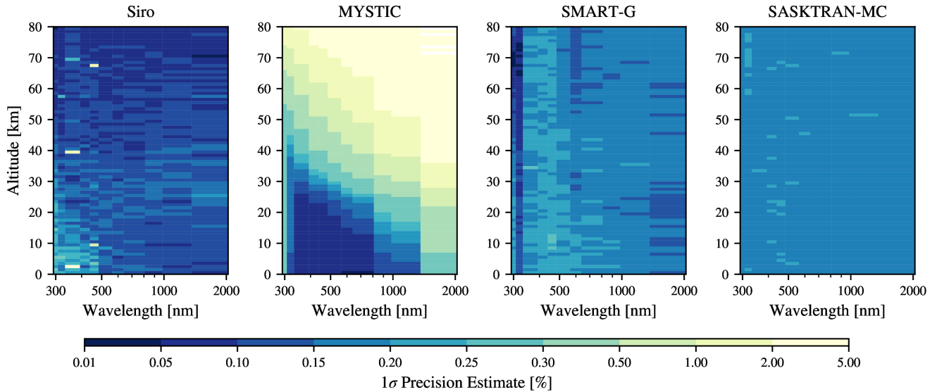
Figure 10. Precision estimates for the MC models with multiple scattering, Rayleigh scattering + ozone absorption + stratospheric aerosol scattering, \text{SZA}=70^\circ , \text{SAA}=30^\circ , and a Lambertian surface reflectance of 1. Precision estimates for MYSTIC, SASKTRAN-MC, and SMART-G were taken from the model output. Siro precision was estimated by running the above scenario 20 times and taking the standard deviation.
