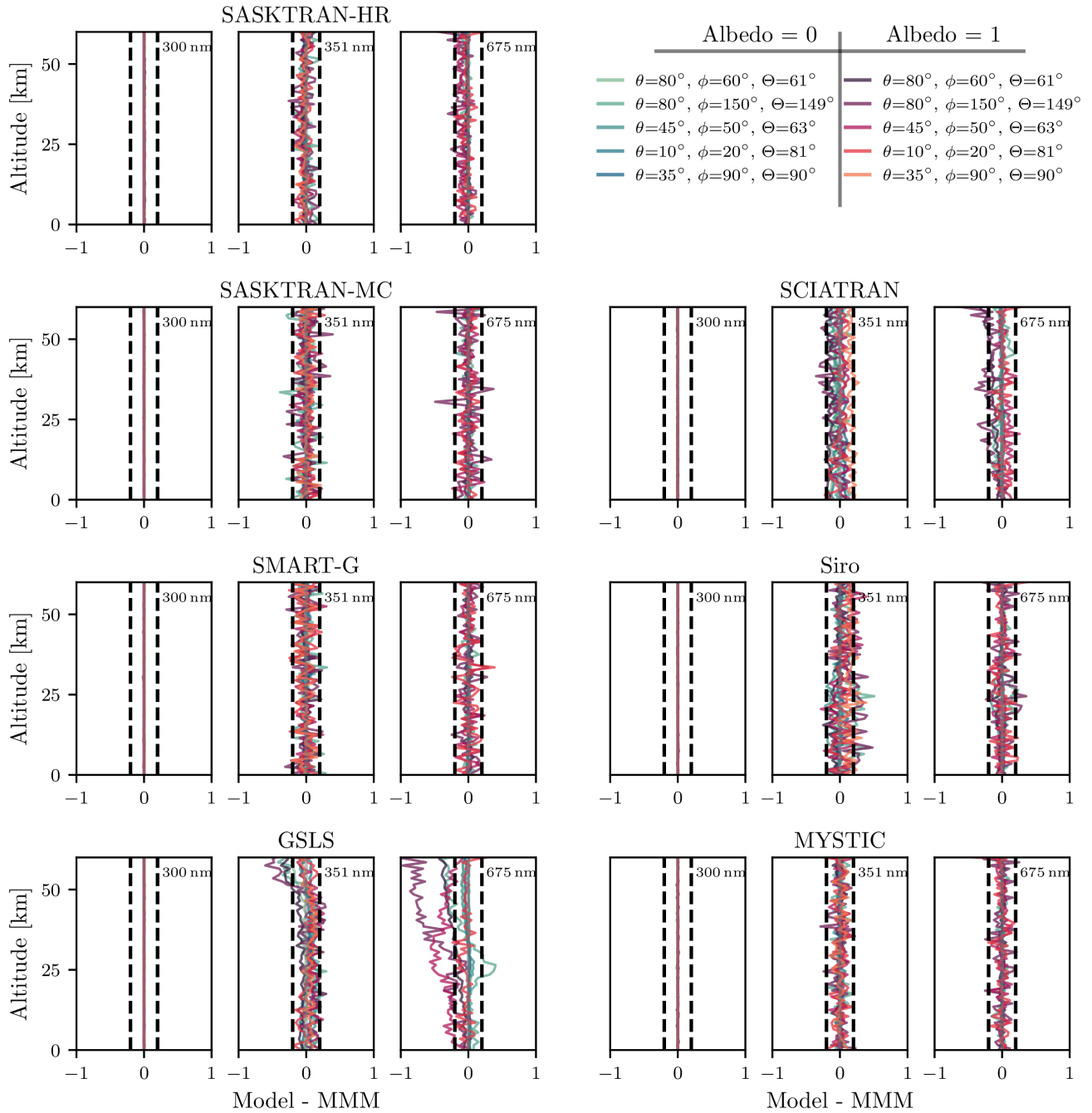
Figure 7. Absolute differences in LPO [°] relative to the MMM (MYSTIC, SASKTRAN-MC, and SMART-G) for each RTM at a variety of wavelengths and solar conditions. The atmospheric optical properties include Rayleigh scattering, ozone absorption, and stratospheric aerosol Mie scattering. Refraction is disabled. Dashed vertical lines indicate \pm 0.2^\circ levels.
