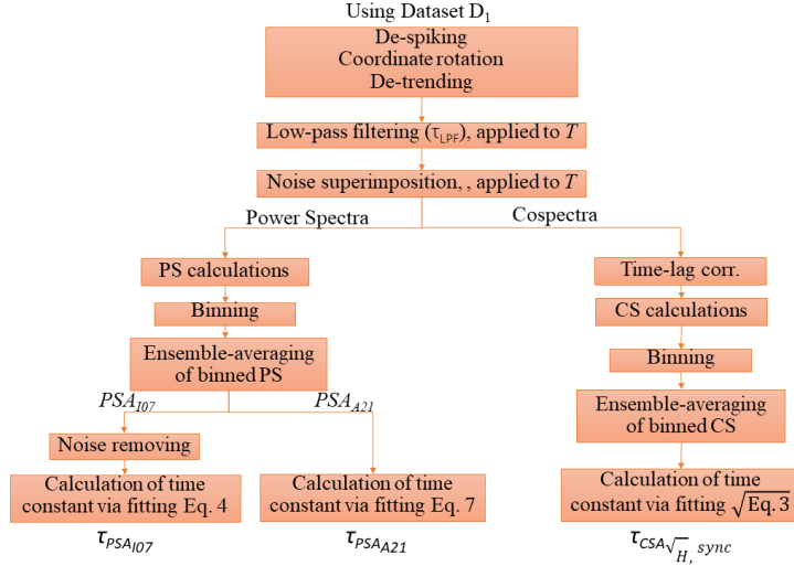
Figure 2. Flow chart of the data processing for time constant calculation using the dataset D_1 . \tau_{LPF} is the time constant of the first order filter. \tau_{PSA_{107}} and \tau_{PSA_{21}} represent the estimated time constants with power spectra (PSA), while \tau_{CSA_{\sqrt{H}, sync}} , \tau_{CSA_{\sqrt{H}}} and \tau_{CSA_H} with cospectra (CSA) approaches. H is the spectral transfer function.
