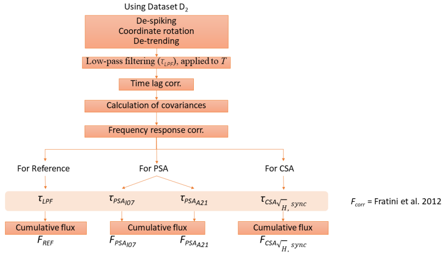
Figure 3. Flow chart of the data processing for the cumulative flux calculation using T of dataset D_2 . F_{REF} refers to reference cumulative flux obtained via frequency response correction applied, where the correction factor ( F_{corr} ) is calculated as the ratio of covariances of unattenuated and attenuated of T and w . F_{PSA_{107}} , F_{PSA_{A20}} , F_{PSA_{A21}} , F_{CSA_{\sqrt{H},sync}} , F_{CSA_{\sqrt{H}}} and F_{CSA_H} F_{REF} are the cumulative fluxes corrected via following Fratini et al. (2012), where F_{corr} is calculated via implementing the time constants (for PSA; \tau_{PSA_{107}} and \tau_{PSA_{A20}} , \tau_{PSA_{A21}} , for CSA; \tau_{CSA_{\sqrt{H},sync}} , \tau_{CSA_{\sqrt{H}}} and \tau_{CSA_H} for reference; \tau_{LPF} ) calculated in previous section.
