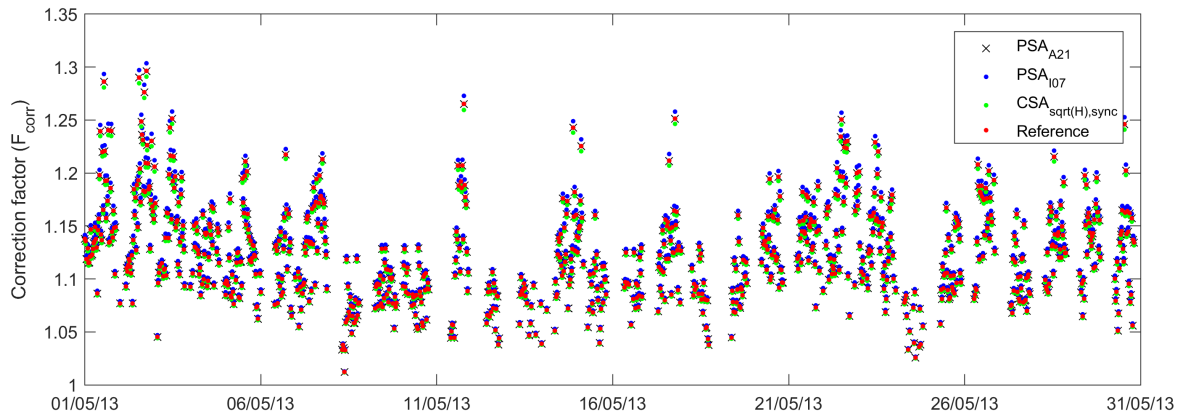
Figure 10. Correction factors ( F_{corr} ) of half-hourly fluxes calculated with different approaches, i.e. PSA_{A21} (black cross), PSA_{107} (blue point), CSA_{\sqrt{H},sync} (green point) and the reference (red point) for the case with \tau = 0.3s and SNR of two.
