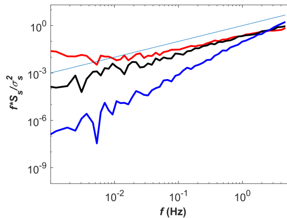
Figure B1. Normalized spectra of methane concentration (red), white noise (black), and blue noise (blue) ( fS_s/\sigma_s^2 ), all of which have the same standard deviation. Solid The solid straight line is f^{+1} line.
