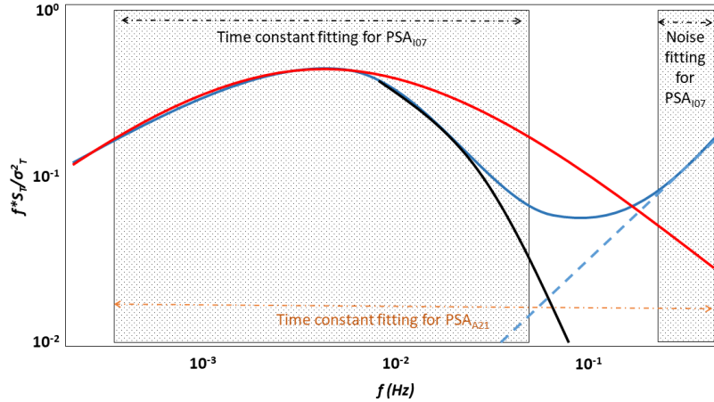
Figure 1. A diagram illustrating two-steps-fitting procedures (i.e. noise removal and transfer function) to estimate time constant for PSA 107 methods. Shown are the spectra of unattenuated and noise-free scalar temperature (red line), and spectra of low-pass filtered and noisy scalar (dark blue solid line) and after (black line) noise removal. The blue-dotted lines are for PSA 107 , the curves fitted noise is detected via fitting a line (blue-dashed) to the high-frequency end of blue line noisy scalar over the frequency range highlighted. Then, then it is extended towards lower frequencies, and subtracted from the noisy spectrum, yielding noise-free spectra. The shaded areas mark Later, the time constant is calculated via fitting Eq. (4) to noise-free spectra over the frequency range used for highlighted. For PSA A21 , the time constant is obtained from one comprehensive fitting for noise removal and transfer function Eq. (7) to noisy spectra over the whole frequency range highlighted.
