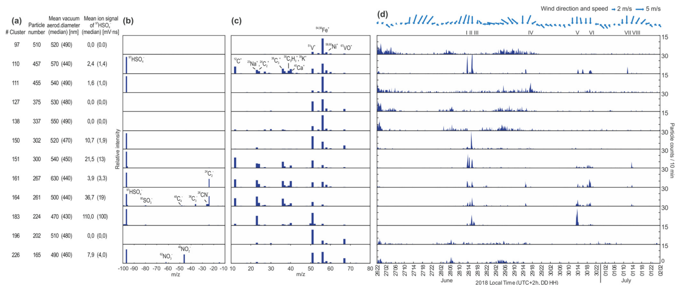
Figure 4: Results of the ART-2a clustering for 12 of the 15 clusters showing signatures of residual fuel combustion. (a) Cluster number according to their labels in the full cluster analysis (see Supplement), particle number, vacuum aerodynamic diameter and average sulfate signal of the clusters. (b) Weight matrices (spectra of the cluster center) of negative ions and (c) positive ions corresponding to average mass spectra. (d) top: measured wind data and ship plume numbers; below: time series of particle counts with 10 min resolution. Note the different y-axis scales. While only mass spectral data was considered in the clustering algorithm, also the time series of the resulting clusters reveal two distinct groups: The transient group with bipolar mass spectra and short events as well as the background group with dominant metal signatures and smooth time series.
