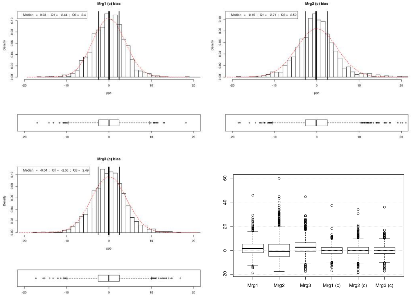
Figure 5. In order from top-left to bottom-right: (A) bias between the reference instrument and the Mrg1 sensor after the LCS correction, (B) bias of the Mrg2 sensor after LCS correction, (C) bias of the Mrg3 sensor after correction and (D) comparison of the LCSs bias before and after correction.
