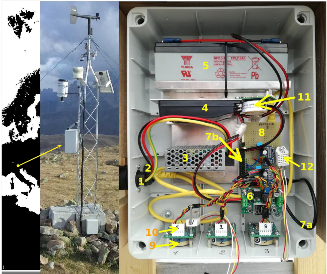
Figure 2. The low-cost sensing system and its components. 1) AC power IN, 2) Ethernet, 3) Power Supply, 4) Charge regulator, 5) Battery, 6) DC/DC converter, 7a) USB power wire, 7b) Raspberry Pi, 8) Data acquisition board, 9) Working sensor, 10) Sensor's plug, 11) Blank sensor, 12) T&RH sensor.
