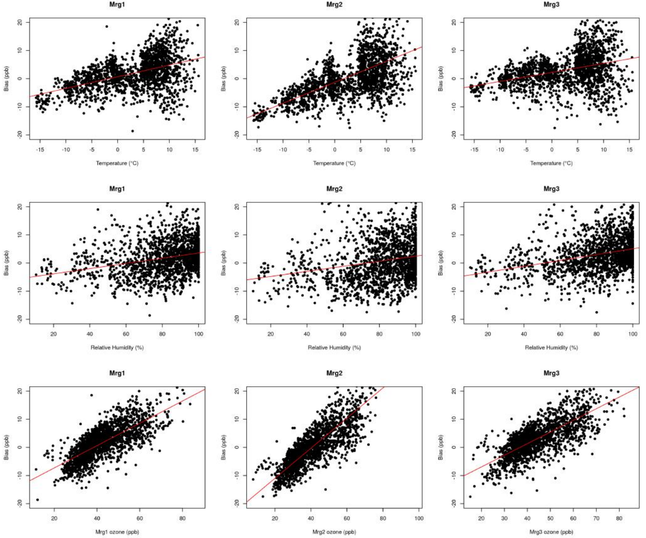
Figure 4. The environmental variables with a non negligible linear correlation with the LCS bias.
