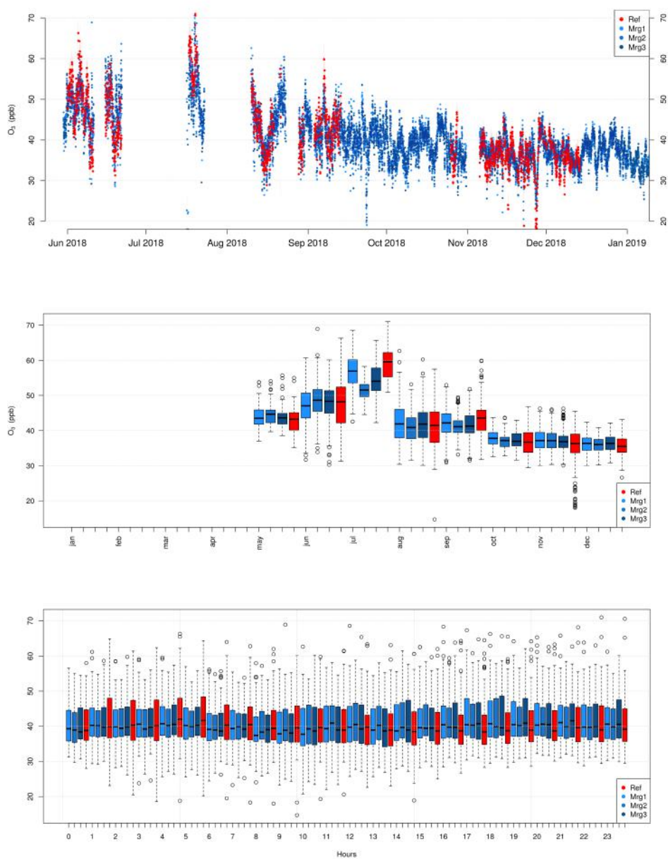
Figure 6. Time series of ozone concentration measurements and meteorological variables for the period June-December 2018. Monthly and hourly boxplots for the period June-December 2018. LCSs average values are reported in blue gradient and the reference ozone concentration is reported in red. Observations from periods where both the LCSs and the reference were operational have been considered for the monthly and hourly boxplots.
