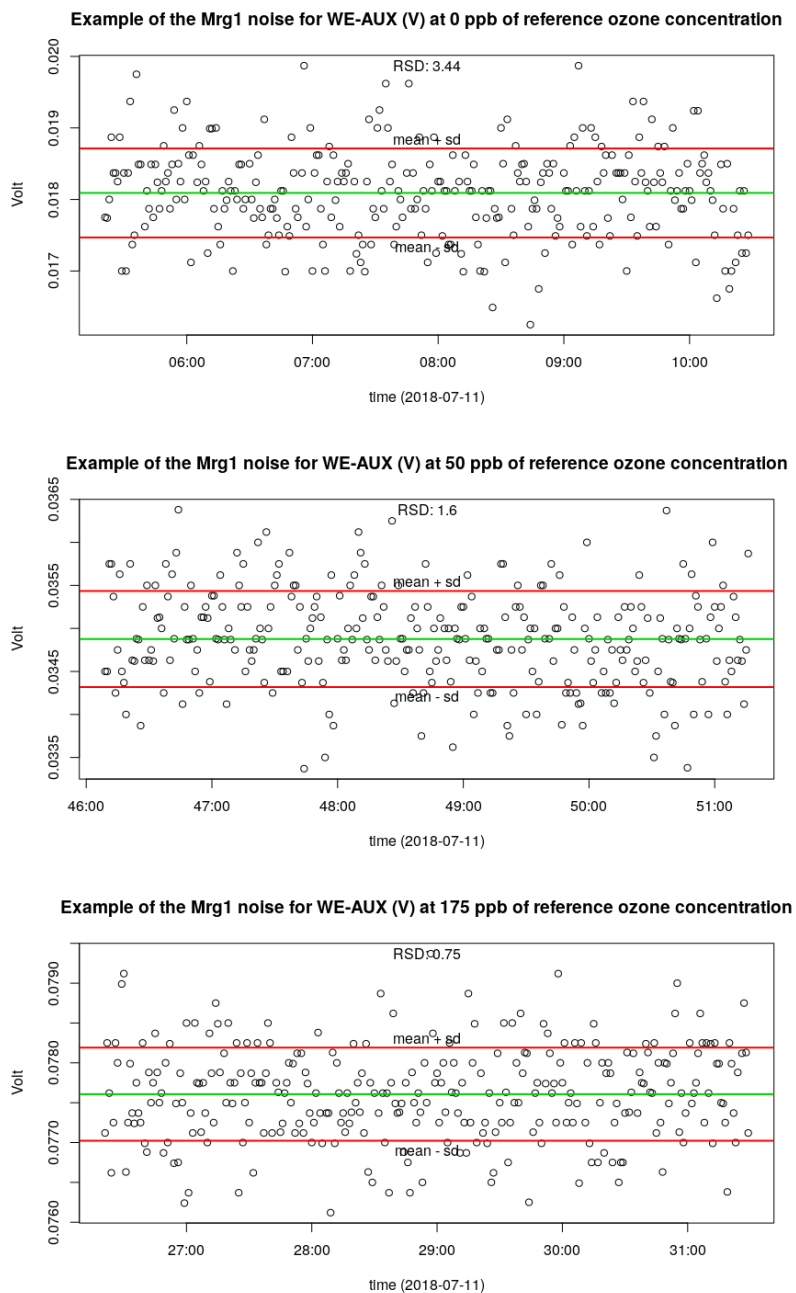
Figure S3.1. Electrical noise of the LCSs.
