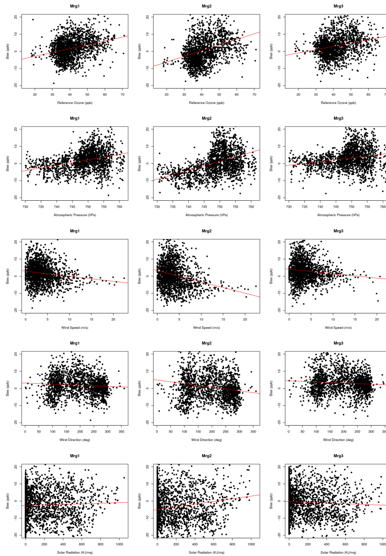
Figure S5.5. Non correlating variables. No evidence of correlation was found among the bias ( O_3^{LCS} - O_3^R ) and the incident solar radiation (PCC \approx 0.05 , p-value \approx 0.1 ), the atmospheric pressure (PCC \approx 0.24 , p-value \approx 0.3 ), the wind speed (PCC \approx -0.22 , p-value \approx 0.1 ) and the wind direction (PCC \approx -0.10 , p-value \approx 0.4 ).
