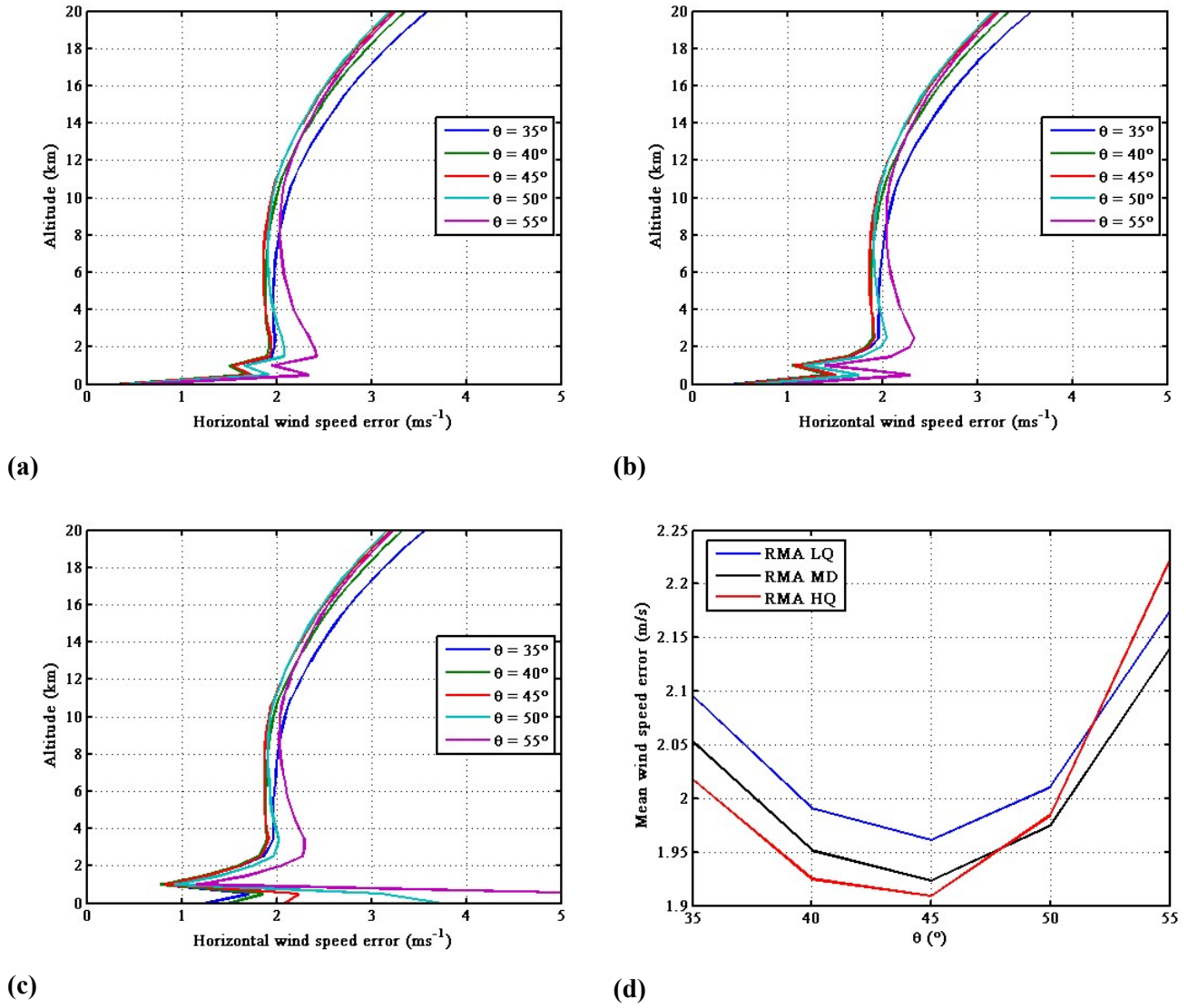
485 Figure 7 (a, b, c) HLOS wind speed statistical error as a function of altitude for LOS angles between 35^\circ and 55^\circ , for Lower Quartile, Median, Higher Quartile RMA aerosols distribution respectively. (d) HLOS wind speed error averaged between 0.5 and 15 km in altitude as a function of LOS angle.
