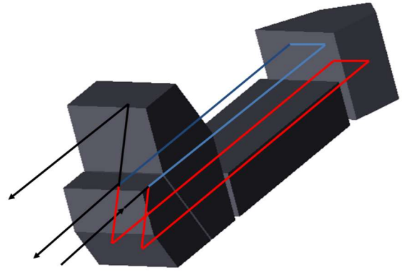
Figure 2 (a) QMZ schematics: BS beam splitter, M mirror, CP field compensation plate, QWP quarter-wave plate, WP Wollaston polarizer, D1, D2 A-CCD detectors; (b) MZ actual prism arrangement (QWP, WP and detectors not shown here).
