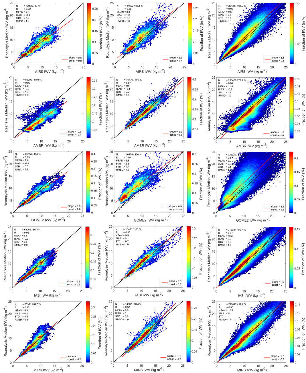
Figure 7. Joint distribution of daily means from the satellite (x-axis; AIRS L2 v6 IR-Only, AMSR, GOME-2, IASI L2 PPFv6, MIRS) and reanalyses median (y-axis CFRSR, ERA-Interim, JRA-55, MERRA2) for the 0.75^\circ \times 0.75^\circ grid points in the Central Arctic (left), Open Ocean (middle) and the full region (right). The time period is May to June 2017. The color indicates the relative fraction of the IWV.
