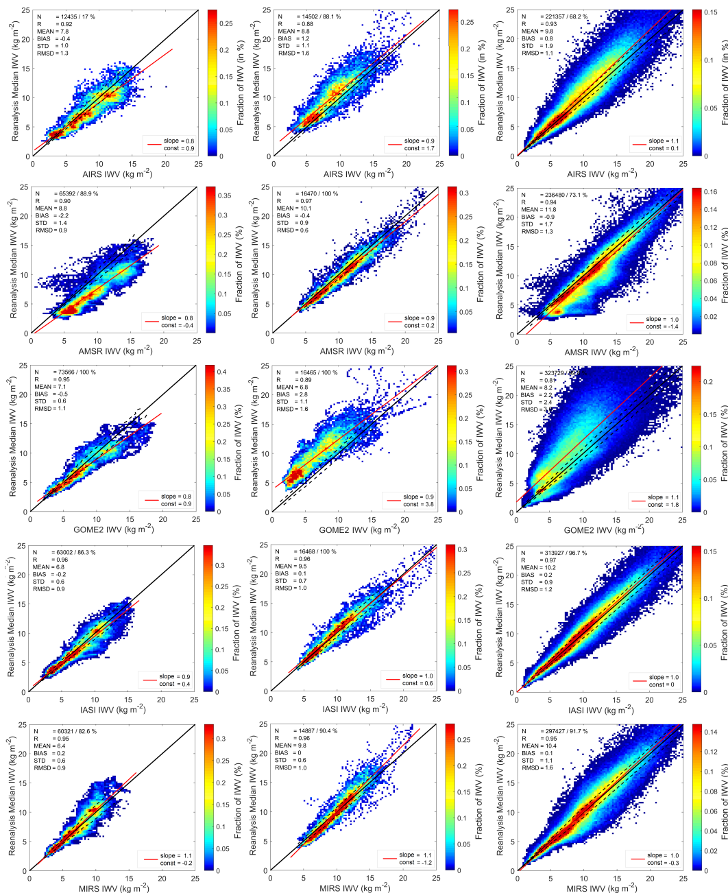
Figure 7. Joint distribution of daily means from the satellite (x-axis; AIRS, AMSR, GOME-2, IASI, MIRS) and reanalyses median (y-axis) CFSR, ERA-Interim, JRA-55, MERRA2) for the 0.75^\circ \times 0.75^\circ grid points in the Central Arctic (left), Open Ocean (middle) and the full region (right). The time period is May to June 2017. The color indicates the relative fraction of the IWV.
