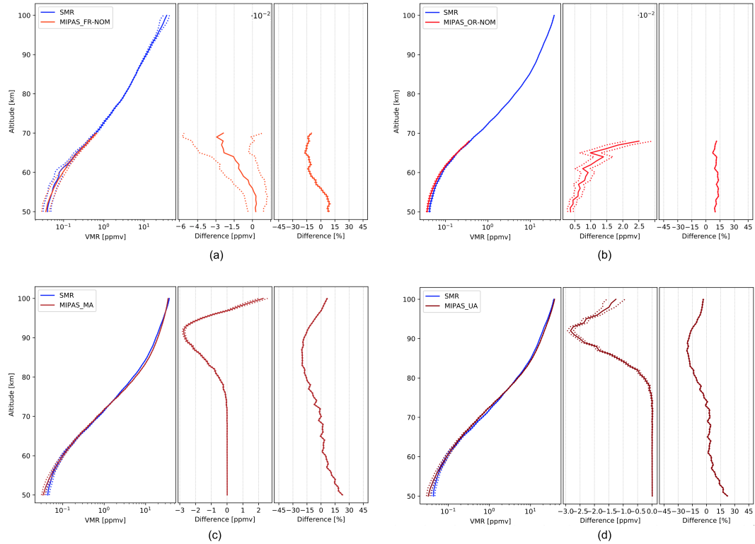
Figure 9. Comparison of SMR CO concentrations with the ones from MIPAS FR-nominal (a), OR-nominal (b), middle atmosphere (c) and upper atmosphere (d) modes. The data plotted are global averages over the whole time periods indicated in Table 2. Left panels: volume mixing ratios, expressed in ppmv. Center panels: absolute differences, expressed in ppmv. Right panels: relative differences, expressed in percentage. The dashed lines represent the standard deviation of the median which, in some cases, is smaller than the thickness of the profile line, causing the dashed line not to be distinguishable.
