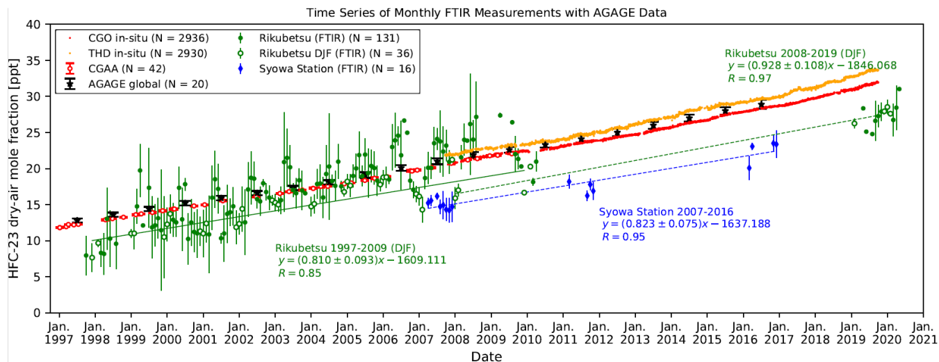
5 Figure 7: Time-series of the monthly mean FTIR-retrieved X_{\text{HFC-23}} at Rikubetsu and Syowa Station, along with the AGAGE in-situ measurements at CGO and THD, and the annual global mean mole fractions and the Cape Grim Air Archive samples, which were reported by Simmonds et al. (2018b).
