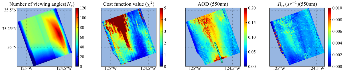
Figure 15. The number of viewing angles used in the retrieval( N_v ), cost function value ( \chi^2 ) and , the retrieved AOD (550 nm) and R_{rs} (550nm) for all pixels in scene 1. Under the condition of N_v > 10 , 94% pixels are available; with \chi^2 < 1.5 , 47% pixels are available; 41% pixels under both conditions. The HSRL AOD AODs at 532 nm are indicated by the colored dots in the AOD plot.
