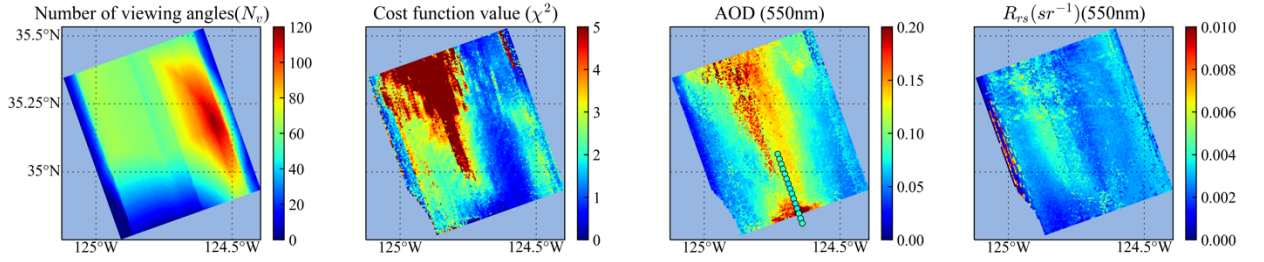
Fig. 15. The number of viewing angles used in the retrieval ( N_v ), cost function value ( \chi^2 ), the retrieved AOD (550 nm) and Rrs (550nm) for all pixels in scene 1. The HSRL AODs at 532 nm are indicated by the colored dots in the AOD plot.
