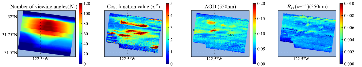
Figure 16. Same as Fig. 15 but for scene 2. For Rrs, viewing angles at least 40^\circ away from the solar specular reflection direction are used to avoid sunglint as shown in Fig. 13.
