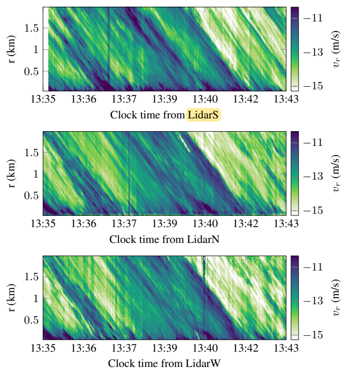
Figure 13. Along-beam velocity component simultaneously recorded on 25-10-2019 by the three scanning lidar instruments at every range gate.
