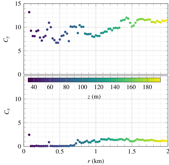
Figure 17. Decay parameters at increasing scanning distances (abscissa) and increasing heights (colorbar) obtained by fitting eq. (7) to the co-coherence between LidarW and LidarN after correction for elevation and azimuth offsets.
