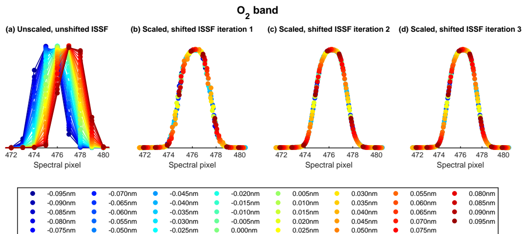
Figure 10. Demonstration of ISSF oversampling for the O 2 band at a central wavelength of 1275 nm and spatial pixel 500. ISSF processing is as described in Figure 9.
