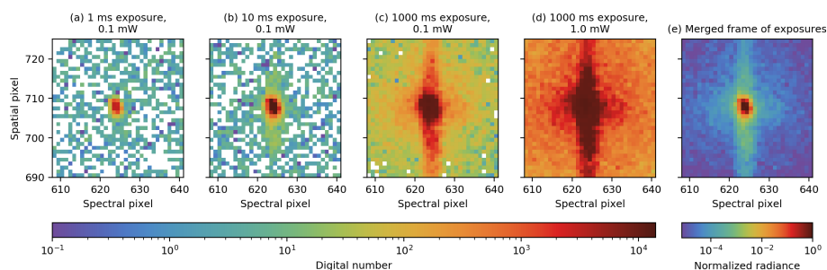
Figure 4. Individual frames with different exposure times in ms and listed laser power in mW (a-d) are combined to create the resulting normalized merged frame (e). At shorter exposure times, the peak is well defined, but the floor is dominated by measurement noise. Longer exposure times allow for characterization of the floor, but the peak and its surrounding area become saturated.
