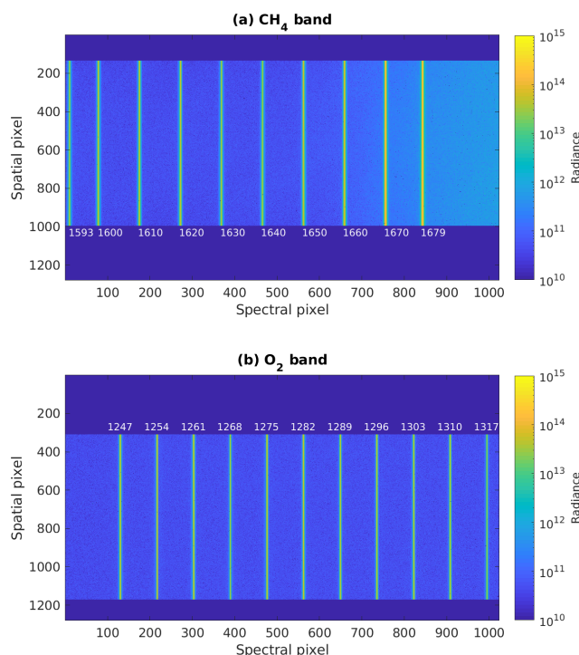
Figure 5. Responses of the focal plane arrays shown as calibrated radiance for the CH 4 (a) and O 2 band (b) over a range of laser wavelengths. The laser wavelengths in nm are labeled next to the corresponding slit images. The radiance is in photons s -1 cm -2 nm -1 sr -1 .
