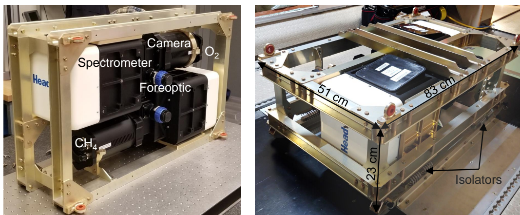
Figure 2. MethaneAIR instrument rack, side view (left) and down-looking configuration in the GV aircraft (right).
