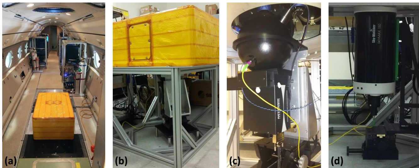
Figure 3. During flight (a) and calibration (b), the instrument is mounted in the same orientation and controlled to the same temperature by the yellow thermal housing. An integrating sphere (c) is used to perform non-uniformity and ISRF calibration, while a collimator (d) is used for stray light measurements.
