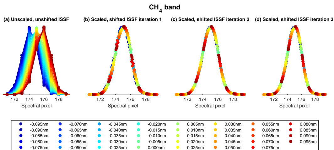
Figure 9. Demonstration of ISSF oversampling for the CH 4 band using a central wavelength of 1610 nm and spatial pixel 500. The laser was scanned in 0.005 nm steps over a range corresponding to the central wavelength ± 0.095 nm. The resulting series of individual ISSFs (a) are then shifted and scaled to produce a single oversampled ISSF (b). Successive iterations of shifting and scaling (c, d) are performed to construct smoother oversampled ISSFs, which can then be mapped from pixel space to wavelength space for ISRF analysis.
