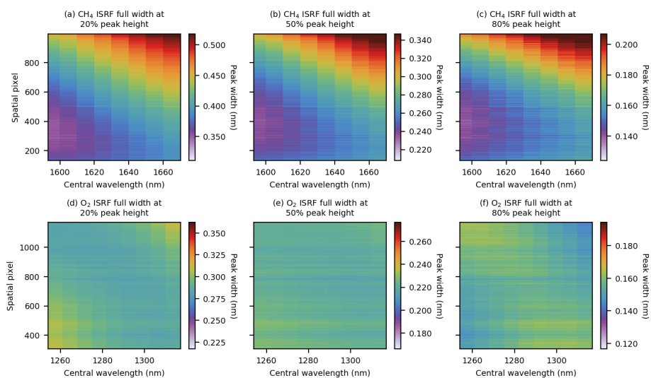
Figure 14. Full width of the smoothed ISRF at 20% (a,d), 50% (b,e), and 80% (c,f) of maximum peak height for all spatial and spectral pixels. The top three panels correspond to the CH 4 band, which shows a general broadening of the ISRF with increasing wavelength and spatial pixel index. In contrast, the O 2 band ISRF is more homogeneous across different spatial and spectral pixels, as reinforced by the relatively narrower scales for the bottom three panels. The color limit in each panel is fixed at \pm 25\% from the FPA-mean value.
