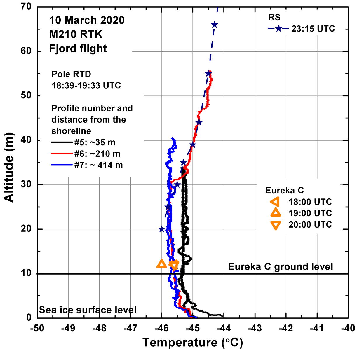
Figure 14. Temperature profiles measured during M210 RTK fjord flight on 10 March 2020 featuring the SBI over the ice covered ocean.
