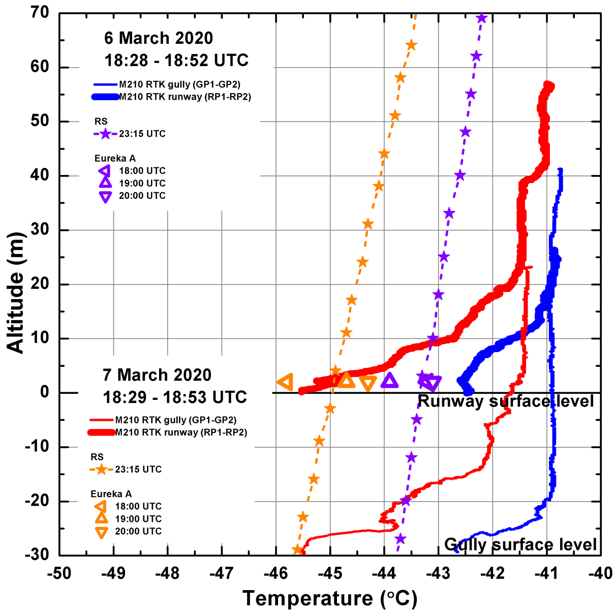
Figure 13. Temperature profiles measured during M210 RTK gully versus runway flights on 6 and 7 March 2020 featuring similar shapes of SBI formed in the gully and above the runway (see Figure 7 for the locations of the temperature profiles).
