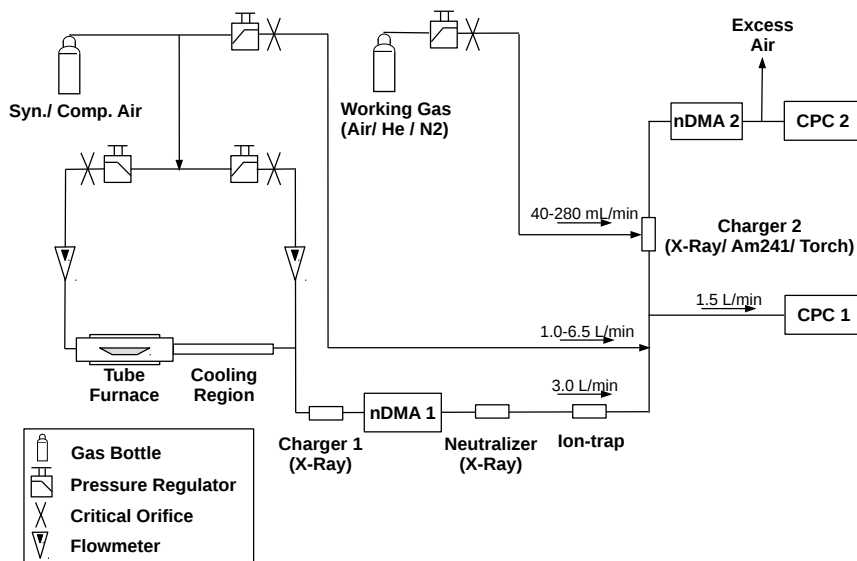
Fig. 2. Schematic of the experimental setup for the charging probability and particle size distribution inversion measurements. The additional working gas flow is only needed for the plasma charger.
