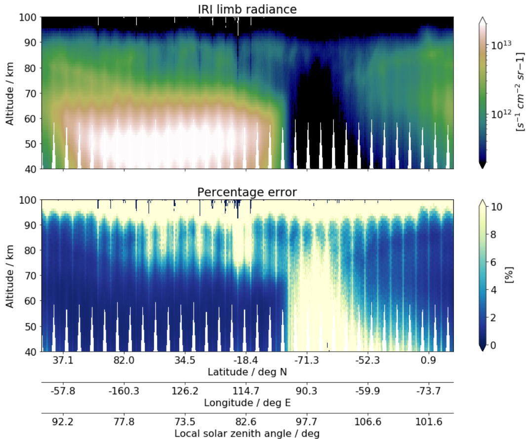
Figure 2. An example of IRI limb radiance data and its percentage error for one orbit collected on 2008-03-30, from 22:21:09 to 23:09:13 (orbit number 38720), as a function of geographical location and tangent altitude. Local solar zenith angle is also shown in the horizontal axis.
