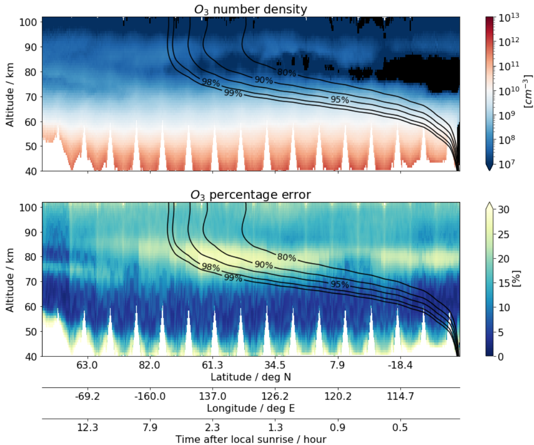
Figure 7. A simple estimation of ozone number density (upper) and its random error relative to the individual a priori profiles (lower), assuming all collected measurements of O_2(a^1\Delta_g) are in equilibrium state, for one orbit collected on 2008-03-30, from 22:21:09 to 23:09:13 (orbit number 38720). Superimposed the contour lines of equilibrium index (see text) corresponding to 80%, 90%, 95%, 98% and 99% of the equilibrium level. Negative values are indicated as black colour. All results shown here have a measurement response greater than 0.8.
