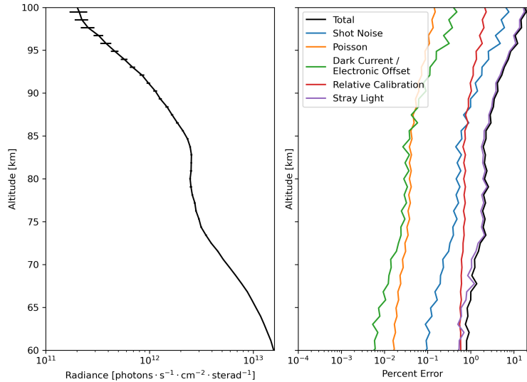
Figure 1. Left: A sample daytime exposure of IRI radiance data (image 1250 of orbit 37400, see Fig. 4 for reference). Right: The corresponding total calibration random error and its contributions.
