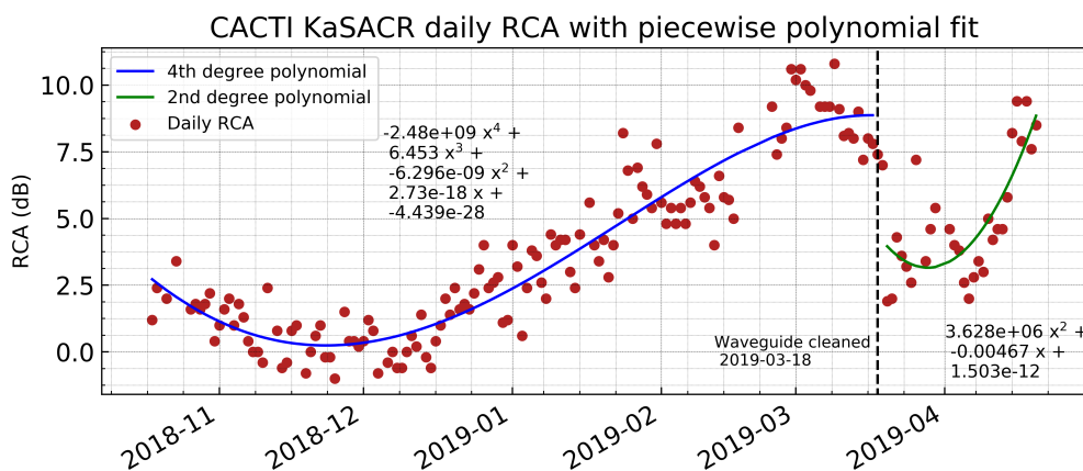
Figure 17. The RCA daily values for the CACTI KaSACR radar are shown with a corresponding piece-wise polynomial fit. A decreasing trend in power resulted in an increasing trend in the RCA value. On March 18th, 2019, the waveguide had an obstruction removed and a sharp decrease (due to corresponding increase in effective power) can be observed. As such a new polynomial fit is calculated for this time period. However, the general trend of decreasing power and increasing RCA continues. The fit is given relative to the epoch time in seconds of each day.
