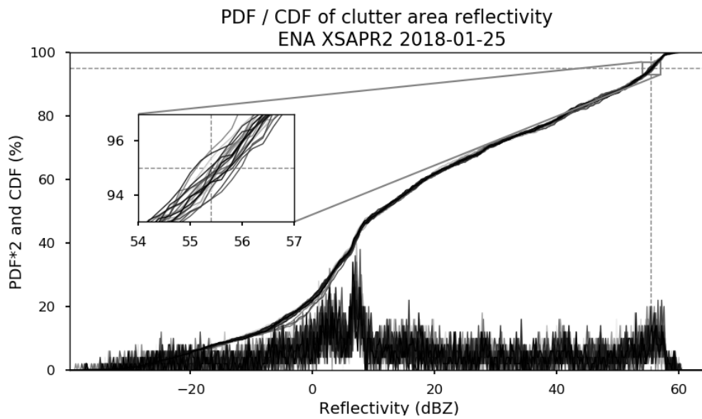
Figure 7. Probability density functions and cumulative distribution functions shown from each hour during the selected baseline day, 25 January 2018, at ENA XSAPR2. The 95th percentile is marked with the corresponding reflectivity value also marked at 55.4 dBZ. This is the value used for the \text{dBZ}_{95_{\text{baseline}}} in the RCA calculation. The inset shows the stability of the 95th percentile for use in the RCA value.
