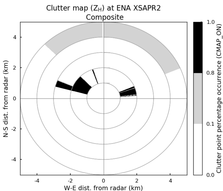
Figure 10. Composite clutter map for XSAPR2 PPIs at the ENA site, created using clutter points from every fifth observation day that occurred at least 80% of the time. The black denotes those time periods that were used for the composite map. The light gray denotes points that made it into a daily clutter map, but were not stable across multiple maps.
