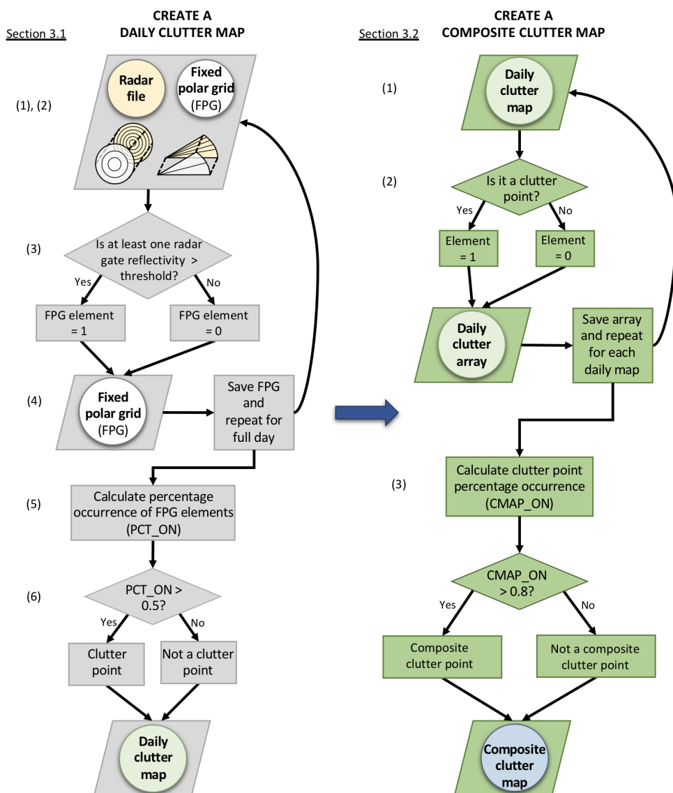
Figure 3. Workflow for designing the clutter map used to calculate the baseline value. The first chart shows how a clutter map is created from a single day of data. The second chart shows how multiple daily maps can be combined into a composite map used in this work that is more resistant to temporal fluctuations.
