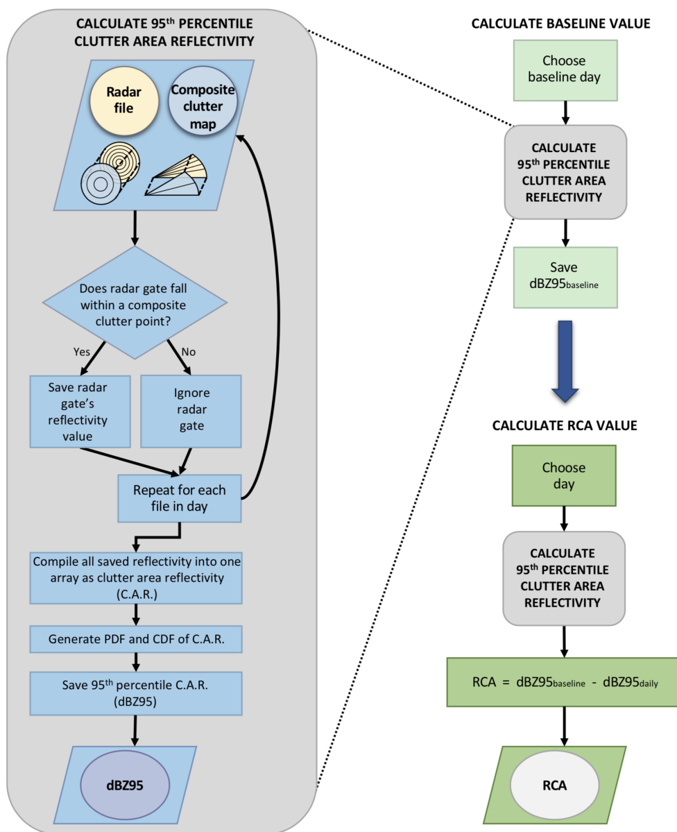
Figure 6. Workflow for calculating a baseline value from the composite clutter map and radar files. The second diagram shows how the baseline value can be used to calculate a daily adjustment to reflectivity.
