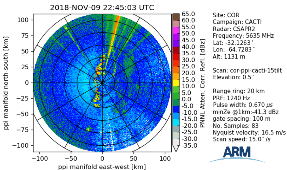
Figure 2. The CACTI CSAPR2 C-band radar PPI from 9 November 2018 22:45:03 UTC. The Sierras de Córdoba lie west of the radar, visible in the ground clutter signature. There is also significant clutter due to the hills to the east of the radar. There are also 3 interference sources visible to the northeast and the northwest. The northwest source is attributable to a transmission tower, while the northeastern is the town of Córdoba.
