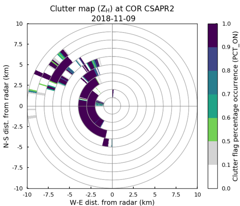
Figure 4. The clutter map calculated from the CACTI CSAPR2 PPI scans on 9 November 2018. The map predominantly uses the clutter caused by the hills to the west of the radar. The clutter to the east of the radar is out of range of the 10 km limit for eRCA.
