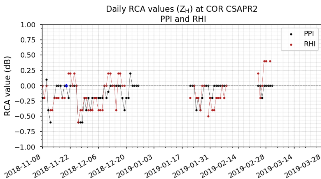
Figure 11. RCA time series for CSAPR2 PPIs and RHIs at the COR site during CACTI. RCA calculated using the composite clutter maps and 20 November 2018 as the baseline. The two radars are within the statistical noise of the eRCA technique. The gaps in the time series are due to periods where the radar was offline.
