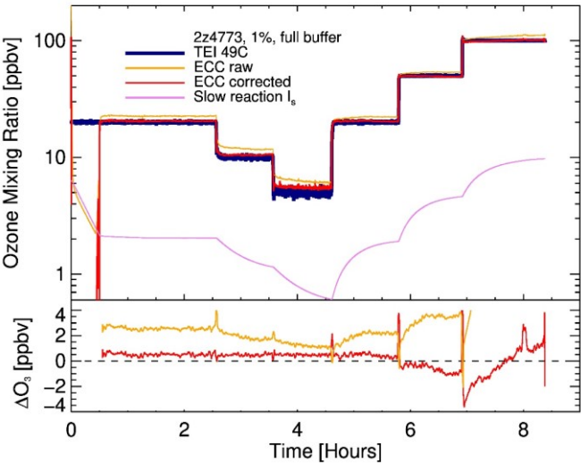
Figure 1: Top: ozone mixing ratio generated by the TEI 49C ozone calibrator (blue) and measured by the ECC (original processing in orange, time response corrected in red). The contribution of the slow reaction is shown in purple. Bottom: difference of raw (orange) and corrected (red) ECC measurements from TEI 49C ozone concentration.
