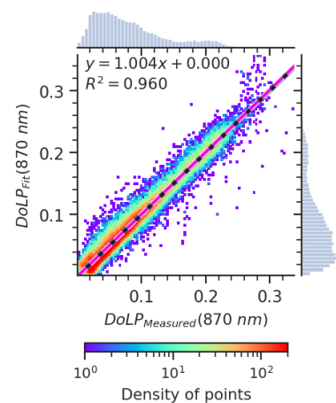
Figure 12. Scatter density plot for AirHARP measurement variables and GRASP fit for the scene in Fig. 9. 1:1 line (black solid line), Ordinary Least Square (OLS) regression line (magenta dashed line), the OLS fit parameters and correlation ( R^2 ) are also reported in the same graph. For each plot, the histogram of measurement and GRASP fit for I and DoLP are plotted on the top and right axis respectively.
