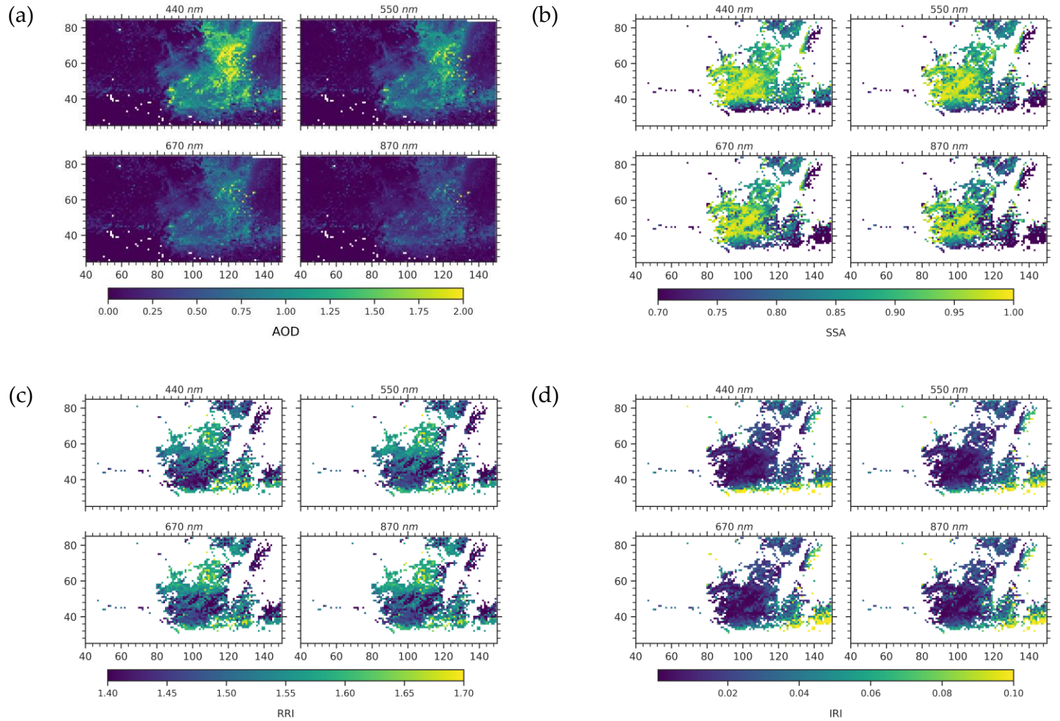
Figure 9. (a) AOD map of a subsetting portion of the 27 th October 2017 T18:16 UTC smoke scene that was marked by a red rectangular box in Fig. 8; (b) Single Scattering Albedo (SSA) for the same subsetting portion in (a) but the pixels with the goodness of fit, \chi^2_{norm} > 5 and AOD_{440\text{ nm}} < 0.4 are masked. (c) same as (b) except the real part of the refractive index (RRI) is plotted. (d) same as (b) except the imaginary part of the refractive index (IRI) is plotted. X and Y axes are the pixel coordinates
