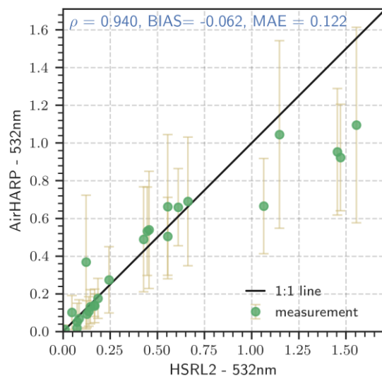
Figure 13. (a) AOD at 532 nm from AirHARP versus HSRL2 AOD at 532 nm along the flight track for the forest fire scene on 9 th November 2017 T19:30 UTC; (b) Correlation plot for the HSRL2 AOD at 532 nm vs AirHARP AOD at 532 nm for the same flight.
