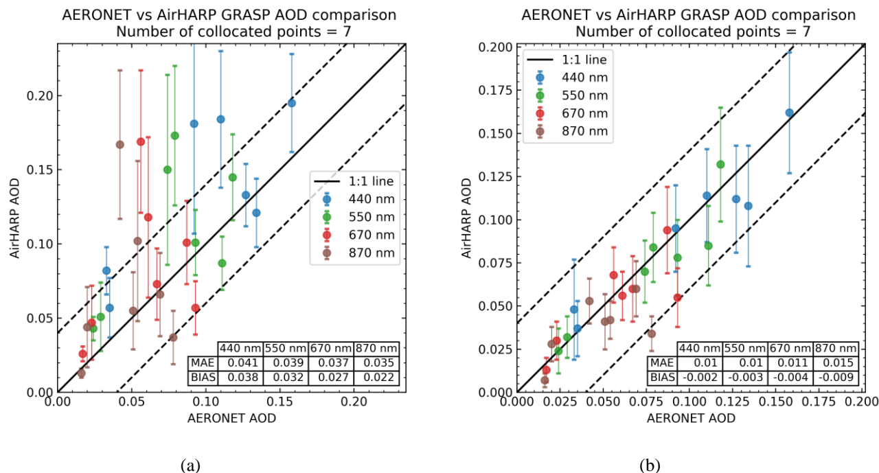
Figure 14. Scattergrams of aerosol optical depth (AOD) retrieved using AirHARP observations over collocated AERONET stations vs AERONET measured AOD interpolated to AirHARP spectral bands. Plotted are the areal mean AirHARP AODs calculated from all the qualified retrievals within a box of 5.5km x 5.5km around the AERONET station against the collocated AERONET temporal mean AOD. Each colored error bar indicates the standard deviation of AOD within the areal box. Mean Absolute Error (MAE) and BIAS for each spectral band are provided in the table inside the scattergram. The black solid lines in the plots are the 1:1 lines and the dashed lines are \pm 0.04 AOD from the 1:1 line. (a) GRASP retrievals using the GRASP/Five mode kernel (Table 3) that has 15 free parameters and allows for retrieval of particle properties along with AOD; (b) same as (a) except using the GRASP/Models kernel (Table 4) that reduces free parameters to 6 and fixes particle properties based on Table 4 and only retrieves the concentration for each aerosol component.
