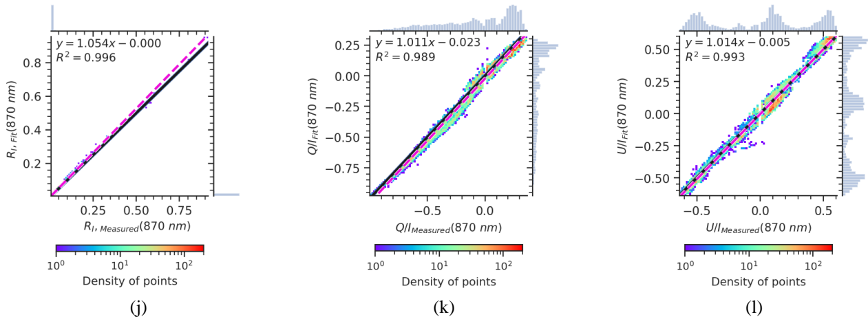
765 Figure 6. Scatter density plots for AirHARP measurement variables and GRASP fit for the ocean scene in Fig. 4(a). The subplots (a), (d), (g) and (j) are the 2D density plots for variable I at different spectral bands blue, green, red and NIR, respectively; (b), (e), (h) and (k) are for the variable Q/I; (c), (f), (i) and (l) are for the variable U/I. The dashed magenta line is the Ordinary Least Square (OLS) Fit for the measured and GRASP fitted variable. The solid black line is the 1:1 line for the measured and fitted variable. 770 There are 72,000 data points for 440, 550, and 870 nm bands and 216,000 data points for the 670 nm band. For each plot, the histogram of measurement and GRASP fit for each variable are plotted on the top and right axis respectively.
