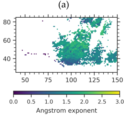
Figure 11. Map of (a) angstrom exponent (AE), (b) aerosol volume concentration, and (c) spherical fraction (SF) of the scene shown in Fig. 9. Pixel filtering similar to the one applied for SSA, RRI, and IRI in Fig. 9 is applied to filter out bad pixels from AE, aerosol volume concentration, and SF map. X and Y axes are the pixel coordinates.
