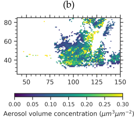
Figure 11. Map of (a) angstrom exponent (AE), (b) aerosol volume concentration, and (c) spherical fraction (SF) of the scene shown in Fig. 9. Pixel filtering similar to the one applied for SSA, RRI, and IRI in Fig. 9 is applied to filter out bad pixels from AE, aerosol volume concentration, and SF map. X and Y axes are the pixel coordinates.
