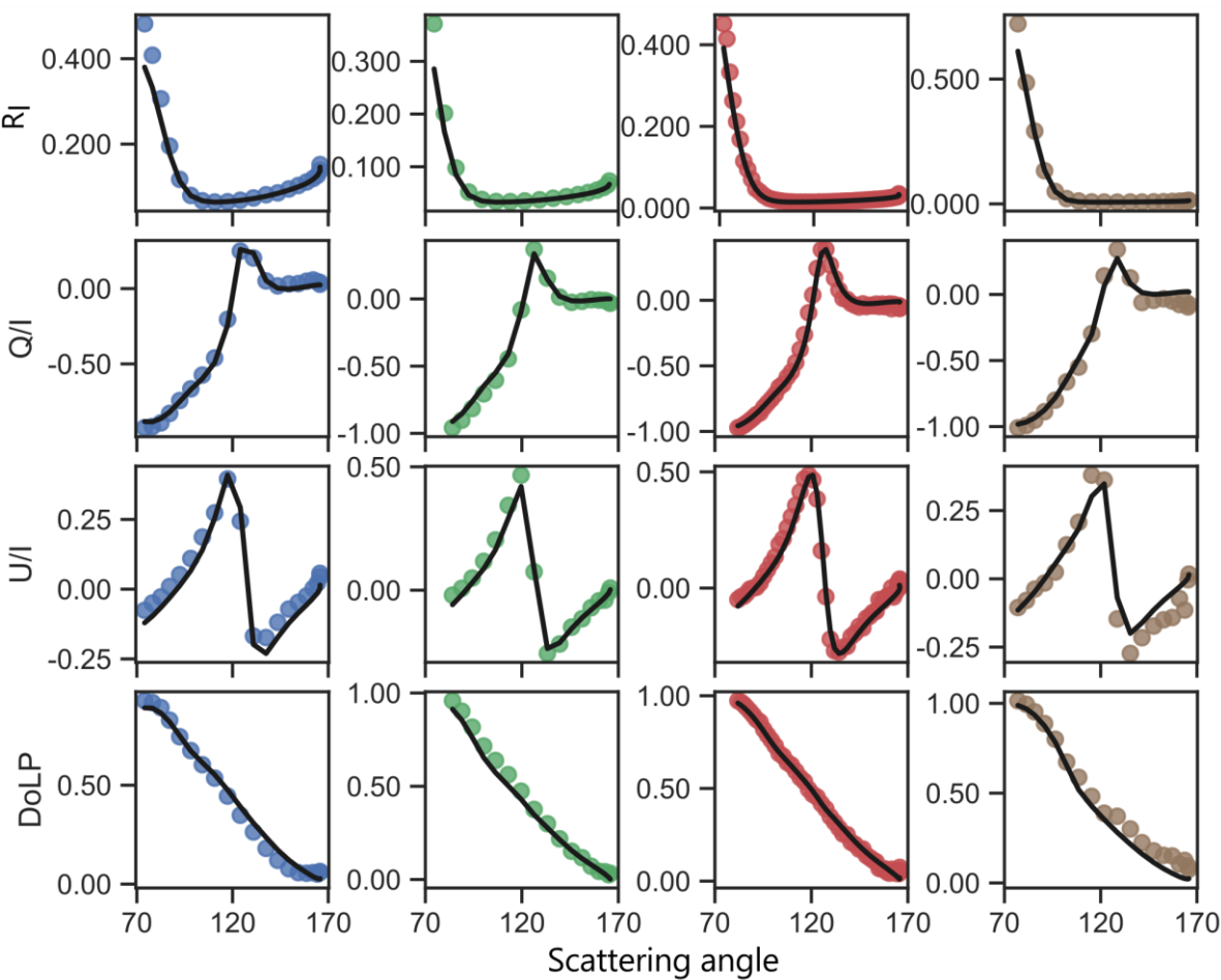
760 Figure 5. AirHARP measured I , Q/I , U/I , and DoLP (solid colored circles) for a single sun glint pixel from the scene in Fig. 4(a) and the GRASP fit to the measurements (black solid line) for all bands (Blue – 440 nm, Green -550 nm, Red – 670 nm and Brown- 870 nm)
