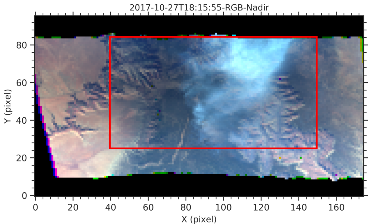
Figure 8. RGB composite image of the 27 th October 2017 T18:16 UTC smoke scene, X, and Y axes are the number of pixels (550m x 550m) along the respective axes. Pixels inside the red rectangular box are used for the aerosol retrievals of AOD, SSA, RRI, IRI. These are plotted in Fig. 9.
