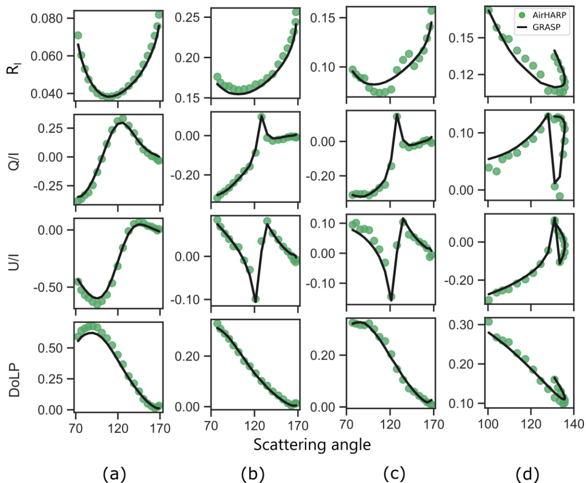
Figure 7. AirHARP measured I, Q/I, U/I, and DoLP (solid colored circles) and the GRASP fit (black solid lines) for selected pixels from the scene in Fig. 4(a,b,c) are plotted for the 550 nm band. Column (a) an offglint pixel from the scene on 23 October 2017 T21:30 UTC; (b) for a dry lake pixel from the flight leg on 25 October 2017 T18:26 UTC; (c) for a vegetation surface also from flight leg on 25 October 2017 T18:26 UTC; (d) for a smoke pixel from flight leg on 27 th October 2017 T18:16 UTC.
