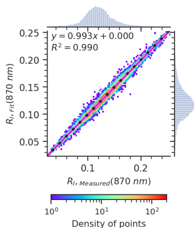
Figure 12. Scatter density plot for AirHARP measurement variables and GRASP fit for the scene in Fig. 9. 1:1 line (black solid line), Ordinary Least Square (OLS) regression line (magenta dashed line), the OLS fit parameters and correlation ( R^2 ) are also reported in the same graph. For each plot, the histogram of measurement and GRASP fit for I and DoLP are plotted on the top and right axis respectively.
