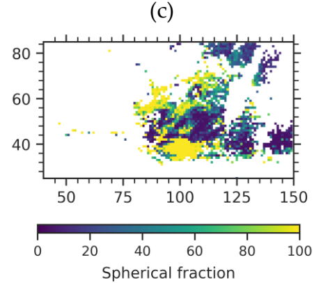
Figure 11. Map of (a) angstrom exponent (AE), (b) aerosol volume concentration, and (c) spherical fraction (SF) of the scene shown in Fig. 9. Pixel filtering similar to the one applied for SSA, RRI, and IRI in Fig. 9 is applied to filter out bad pixels from AE, aerosol volume concentration, and SF map. X and Y axes are the pixel coordinates.
