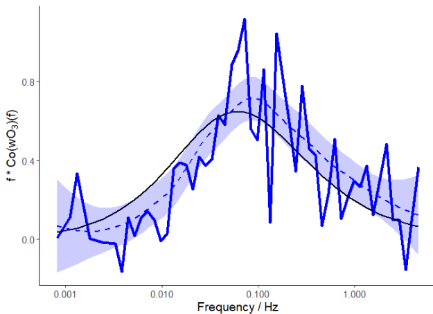
755 Figure 11: Average ozone flux co-spectrum for the 17 th April, normalised to area = 1, shown in blue with a smoothed local regression (LOESS, dashed line) and 95% confidence interval (blue shading). Wind speeds were 10.3 – 12.3 m s -1 and dimensionless Obukhov lengths were 0.14 – 0.17, representing near neutral, slightly stable conditions. Expected co-spectral shape predicted by Kaimal et al. (1972) shown in black.
