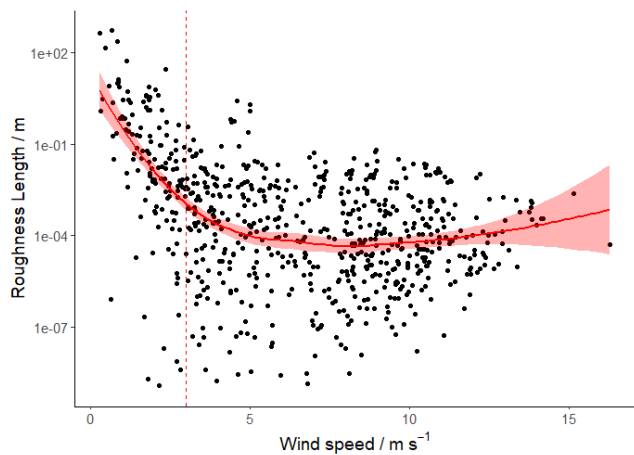
720 Figure 5: Roughness length for each averaging interval (black dots) with a smoothed local regression (LOESS) line (solid red, 95% confidence interval shaded). Points left of the 3 m s -1 filter threshold (dashed red) are not used in subsequent discussions of oceanic deposition velocity. Y axis limited for clarity, with 17 points < 10 -9 m not shown.
