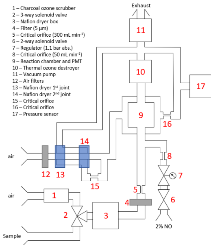
Figure 2: Schematic of the ozone chemiluminescence detector.
