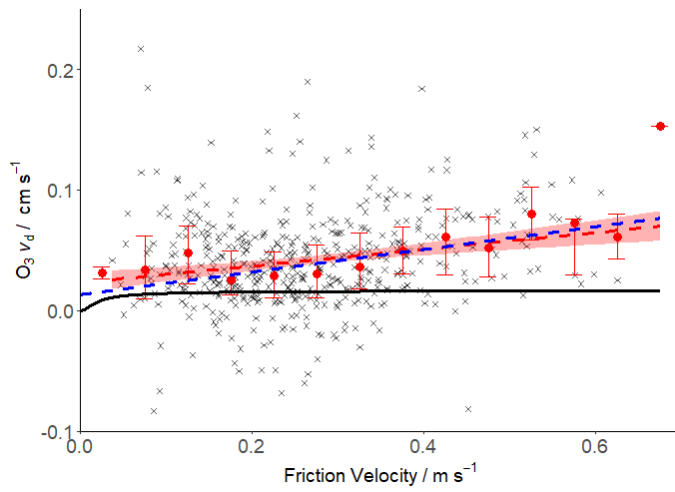
760 Figure 12: Deposition velocity dependence on friction velocity. 20-minute values are shown in grey. Bin-averaged median fluxes (0.05 m s -1 bins) are presented with interquartile ranges in red. Dependence of O 3 deposition velocity on friction velocity is presented with a linear fit in red (95% confidence interval shaded), with the dependence predicted by Fairall et al. (2007) in blue, and that predicted by Luhar et al. (2018) in black.
