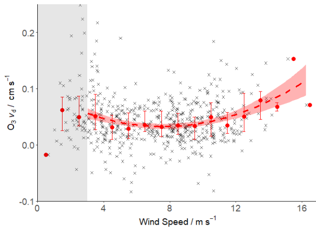
740 Figure 8: Deposition velocity dependence on wind speed. 20-minute values are shown in grey, with bin-averaged medians (1 m s -1 ) and interquartile ranges shown as red dots with bars. A 2 nd order polynomial fit is plotted as a dotted red line with a 95% confidence interval (red shaded area). The grey region below 3 m s -1 indicates values removed by the wind speed filter (Sect. 2.4) that are not included in the fit.
