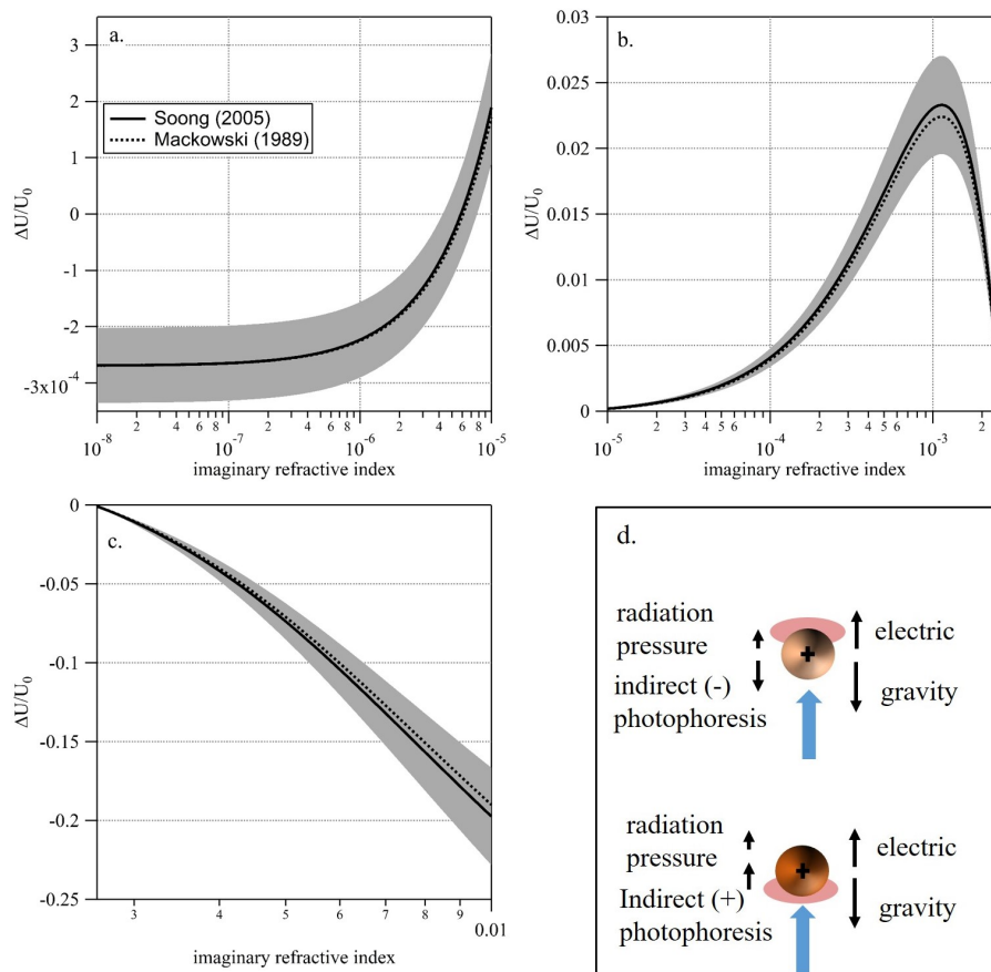
Fig. 1. simulated signal (and uncertainty) for a PEG400 particle, 10 \mu\text{m} in radius at T = 20 \text{ C} , P = 400 \text{ mbar} , m_1 = 1.466 , \lambda = 473 \text{ nm} , I = 35 \text{ mW mm}^{-2} and full thermal accommodation.
