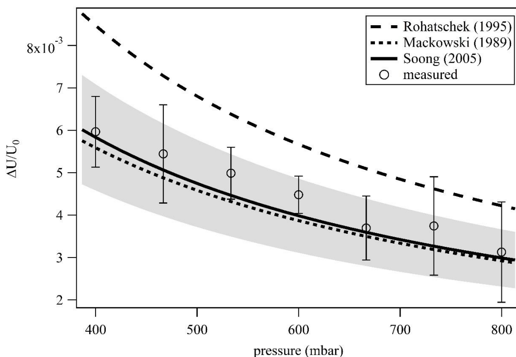
Figure 4. Measured and simulated EDB response ( \Delta U/U_0 ) to the illumination of a slightly absorbing particle due to the photophoretic effect. The two analytical solutions; Mackowski (1989) dotted line and Soong et al. (2005) solid line, that account for slip-flow conditions agree well with our measurements (empty circles). Error bars: standard deviation over five illumination cycles. Gray shaded area: measurement uncertainty propagated through the Soong model calculation, dominated by the 15% uncertainty on the radiant flux measured with a power meter and a beam profiler.
