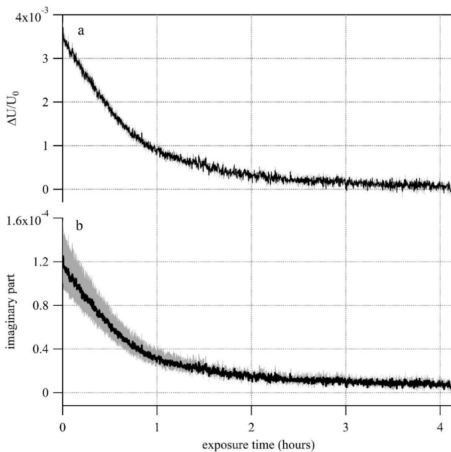
550 Figure 5. (a) Decay of the EDB photophoretic response ( \Delta U/U_0 ) during illumination of a slightly absorbing particle (PEG400 with 0.23% wt of carminic acid; CA). The decay is due to the slow photolysis of the CA. (b) The retrieved imaginary part of the complex refractive index. Gray shaded area in both plots represents the uncertainty in the measured and retrieved values.
