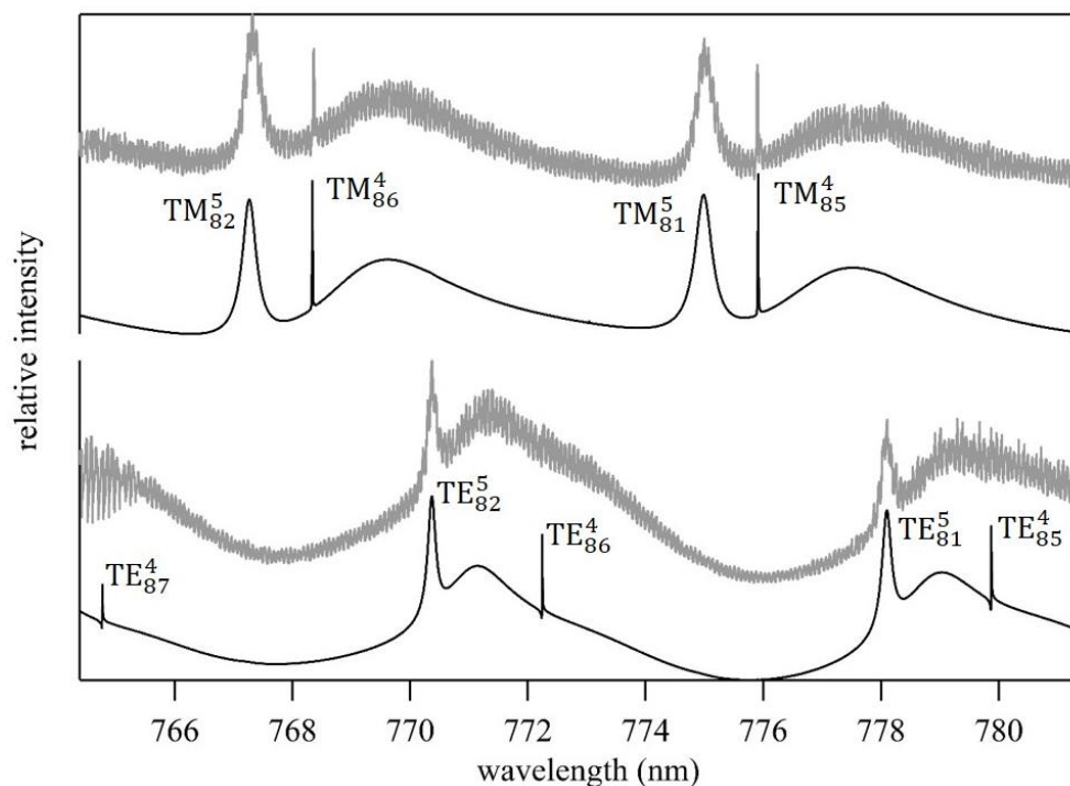
Figure 3. Measured Mie scattering spectra at \pi/2 angle of a levitated particle. The positions of the TE and TM resonance modes (e.g. TM_n^l ; identified by their order ( l ) and mode ( n ) numbers) were used to retrieve the particle's real refractive index ( n_D = 1.4665 , m_1 = 2745 ) and size ( a = 9.2906 \mu\text{m} ). We note that the lower order modes in the fitted TE spectrum are too narrow to be observed in the measured spectrum with the current resolution.
