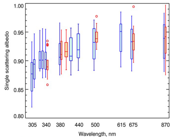
Figure 9. Combined spectral SSA from AMP retrievals (blue symbols) and SKYNET retrievals (orange symbols) using MODIS-derived surface albedo. The bottom and top edges of the boxes are located at the sample 25th and 75th percentiles; the whiskers extend to the minimal and maximal values within 1.5 IQR (interquartile range). The outliers are shown in circles. The center horizontal lines are drawn at the median values. The whisker boxes are computed using AOD_{440} \geq 0.4 criteria to correspond to the best quality level 2 AERONET data. Cited from Mok et al. (2018).
