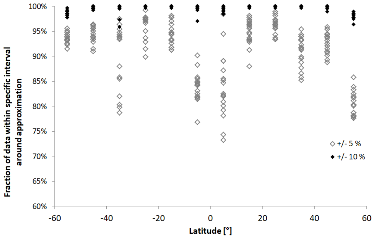
Figure 7 Fraction of data within +/- 5 % and +/- 10 % intervals around approximation.
