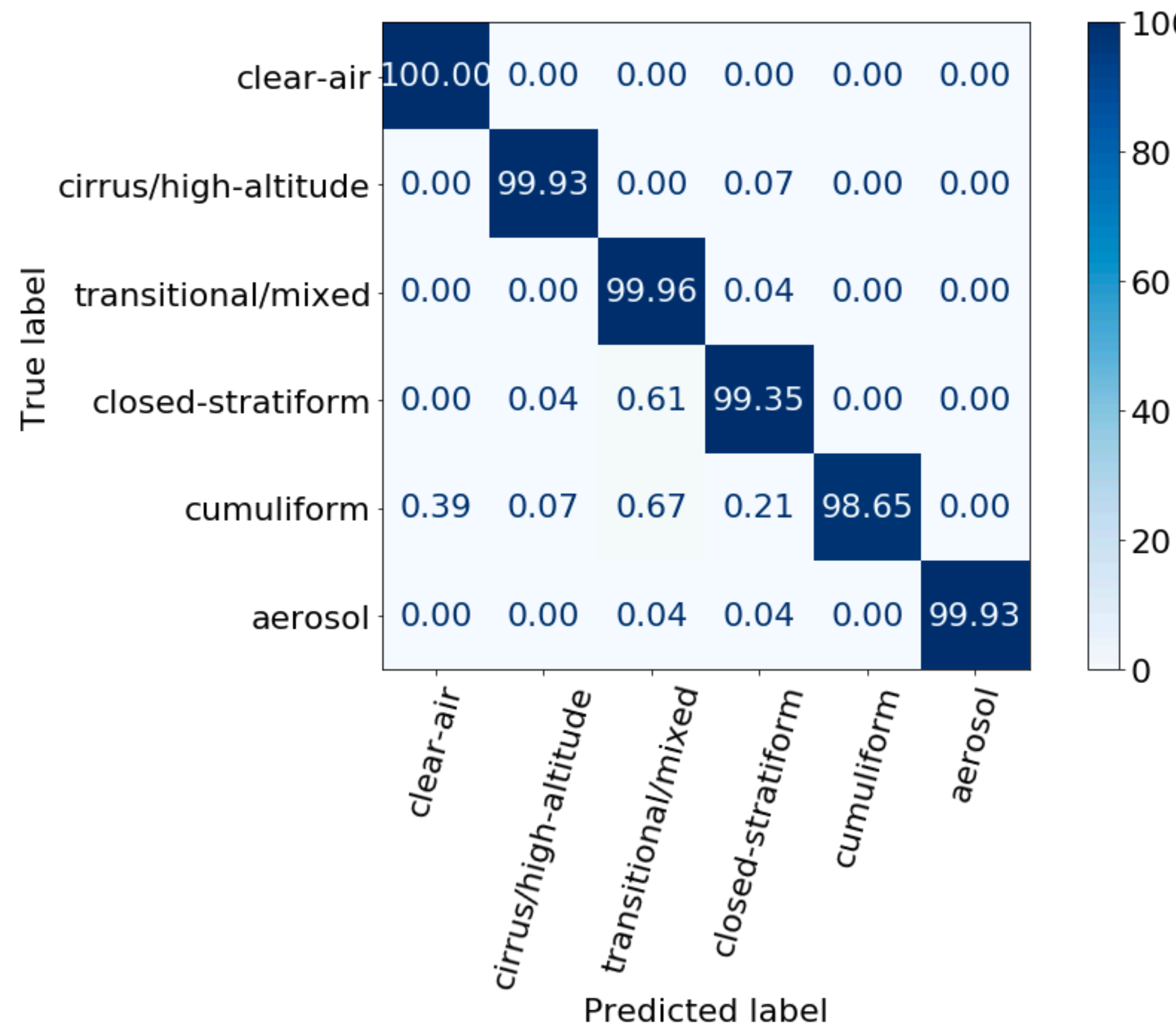
MeanStd A100
