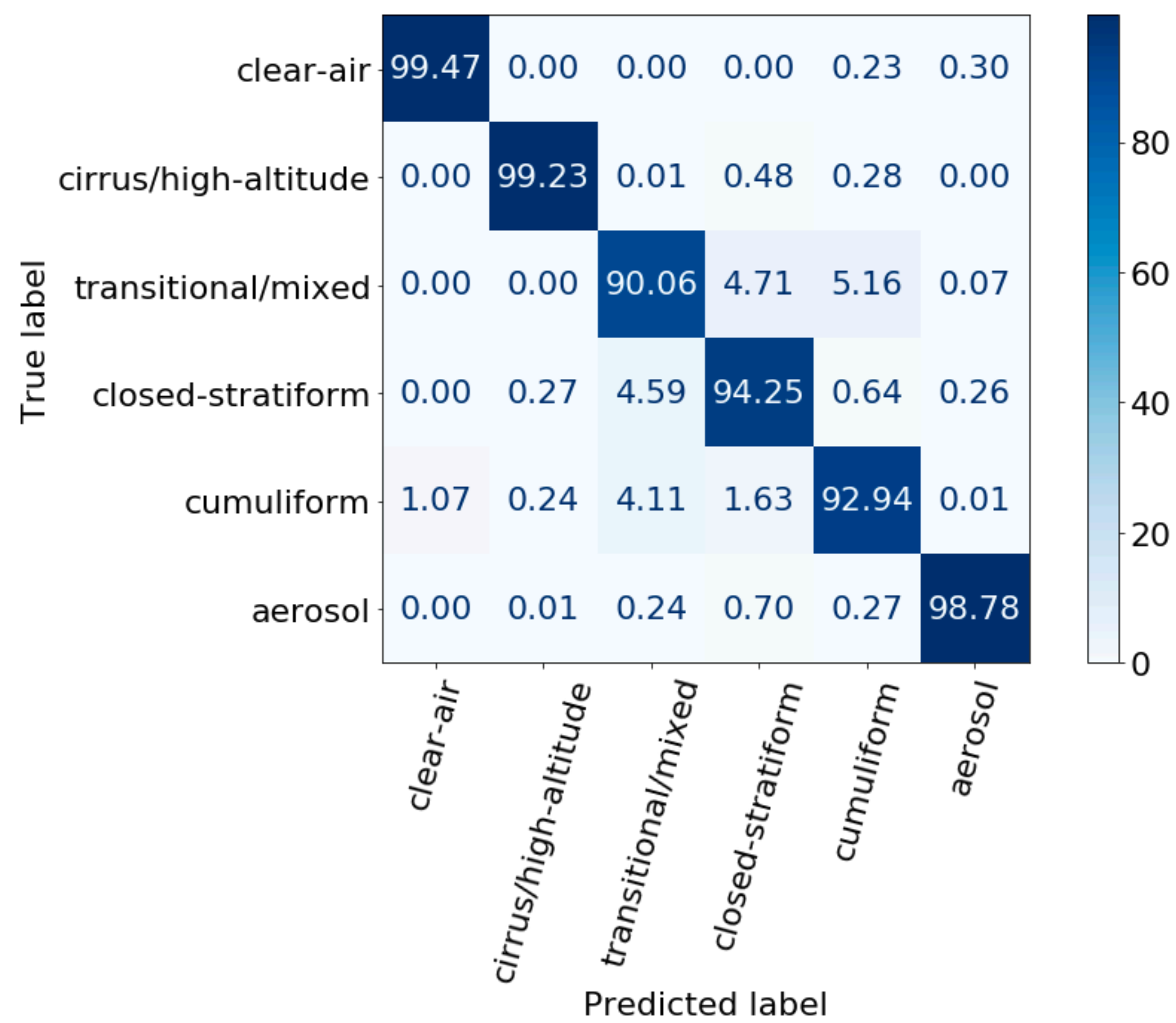
MeanStd A025
