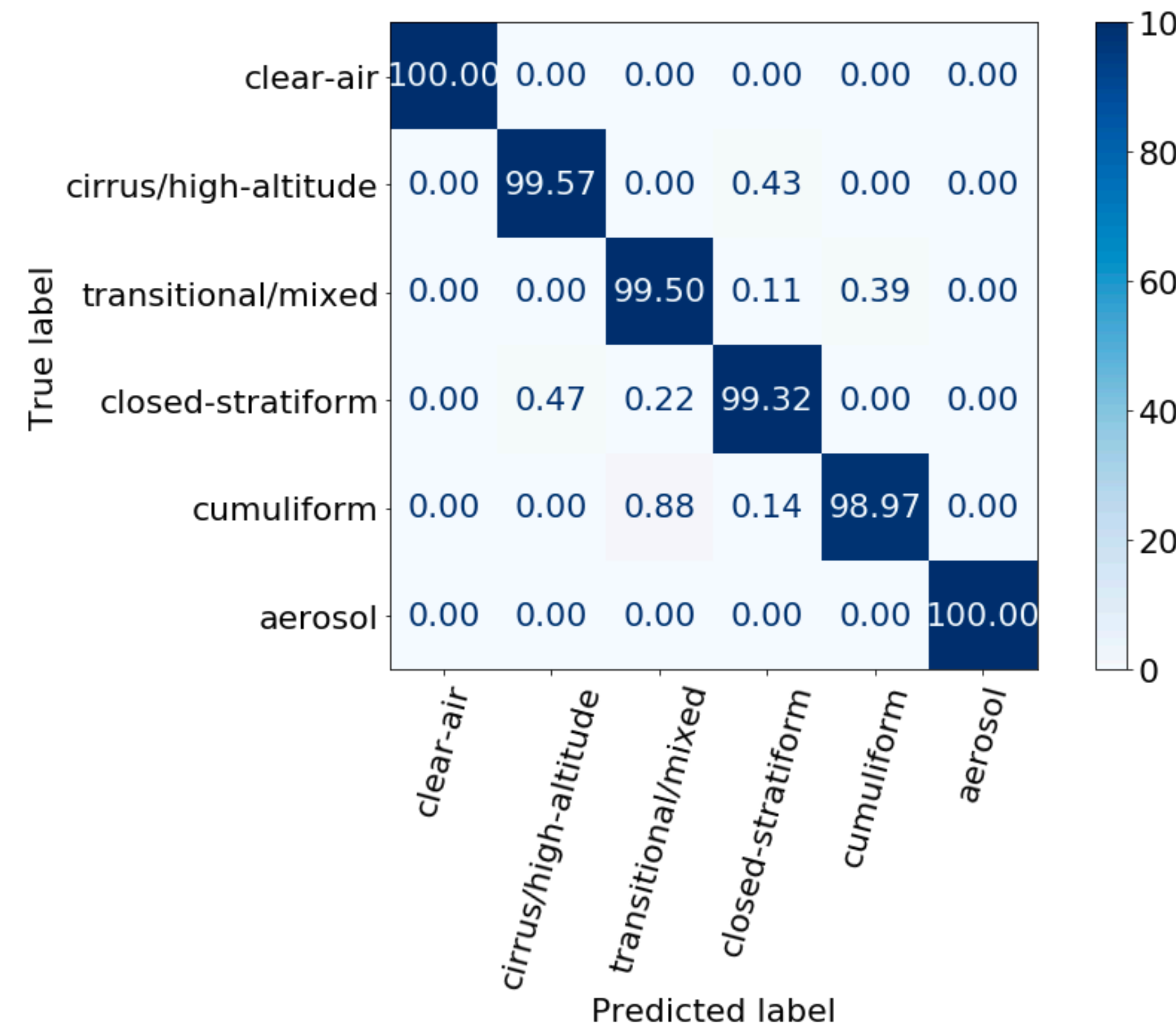
P-CNN A100
