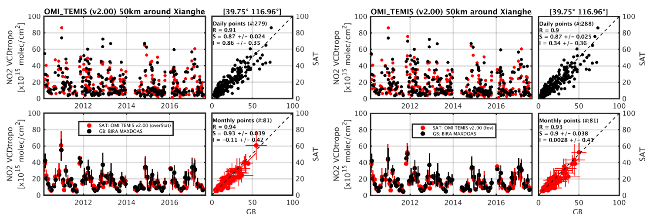
Figure 1. Daily and monthly comparisons at Xianghe when considering only pixels over the station (left), and pixels that crosses the MAX-DOAS field-of-view (right).
