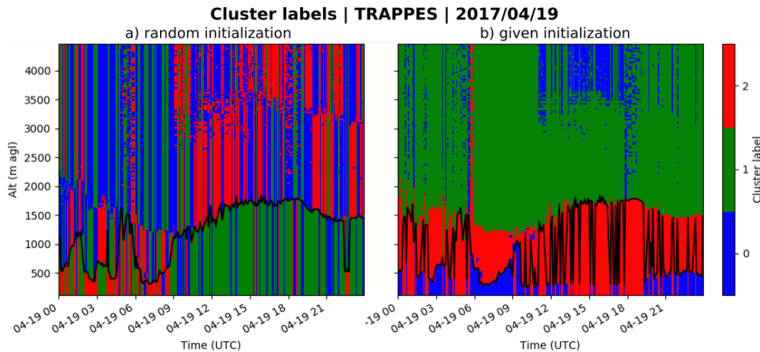
Figure 12. Cluster labels in output of KABL on a time–altitude grid for April 19, 2017, at the Trappes site with the BLH estimated with KABL (black line) with (a) the centroids initialized at random and (b) the centroids initialized at given values.
