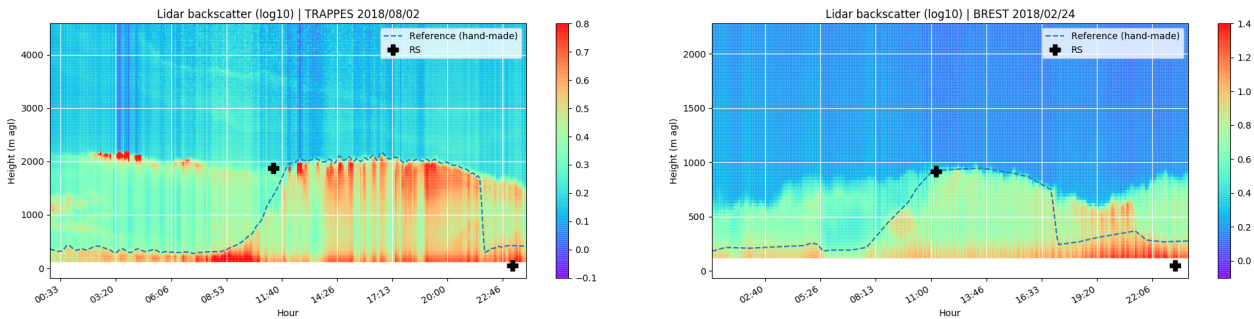
Figure 4. Hand-drawn references and radiosonde estimates overlaying the lidar range-corrected intensity -signal for two days: August 2, 2018, at the Trappes site (left) and February 24, 2018, at the Brest site (right).
