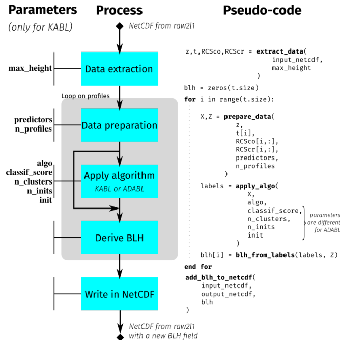
Figure 6. Simplified flowchart of the K-means for Atmospheric Boundary Layer (KABL algorithm) and AdaBoost for Atmospheric Boundary Layer (ADABL) algorithms with a focus on the KABL parameters. The parameters are described in Sect. 3.3 and in Table 2.
