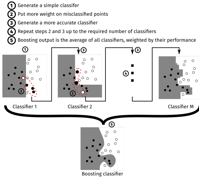
Figure 3. Illustration of boosting on two-dimensional artificial data with two classes.
