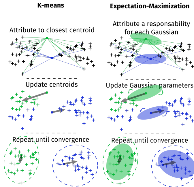
Figure 5. Illustration of the K-means and expectation-maximisation expectation-maximization algorithm on two-dimensional artificial data and with two clusters.
