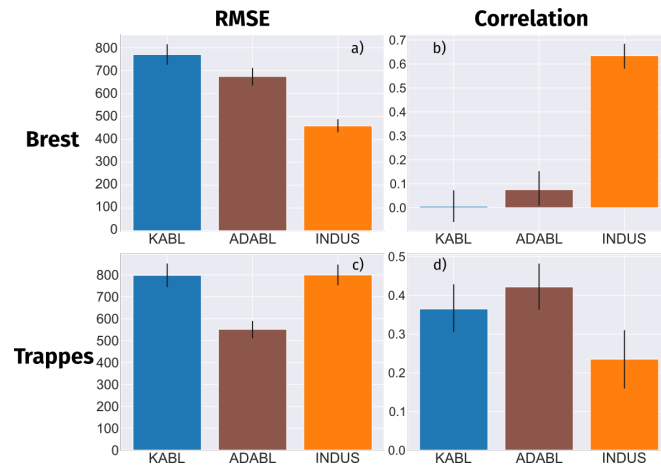
Figure 9. Results of a two-year comparison with the radiosonde (RS) estimates at both sites for two metrics: RMSE and correlation. Cases at night or with rain, fog, an RS-estimated boundary layer height (BLH) of under 120 m, or clouds under 3000 m were removed. The 95% confidence intervals were estimated using percentile bootstrapping (Davison and Hinkley, 1997).
