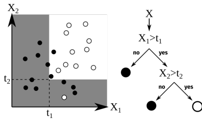
Figure 2. Illustration of binary classification with decision trees on two-dimensional artificial data.
