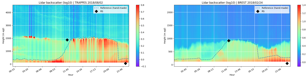
Figure 4. Hand-drawn references and radiosonde estimates overlaying the lidar range-corrected signal for two days: August 2, 2018, at the Trappes site (left) and February 24, 2018, at the Brest site (right).
