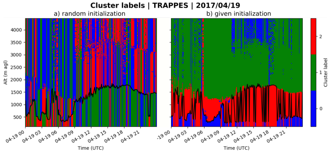
Figure 12. Cluster labels in output of KABL on a time–altitude grid for April 19, 2017, at the Trappes site with the BLH estimated with KABL (black line) with (a) the centroids initialized at random and (b) the centroids initialized at given values.
