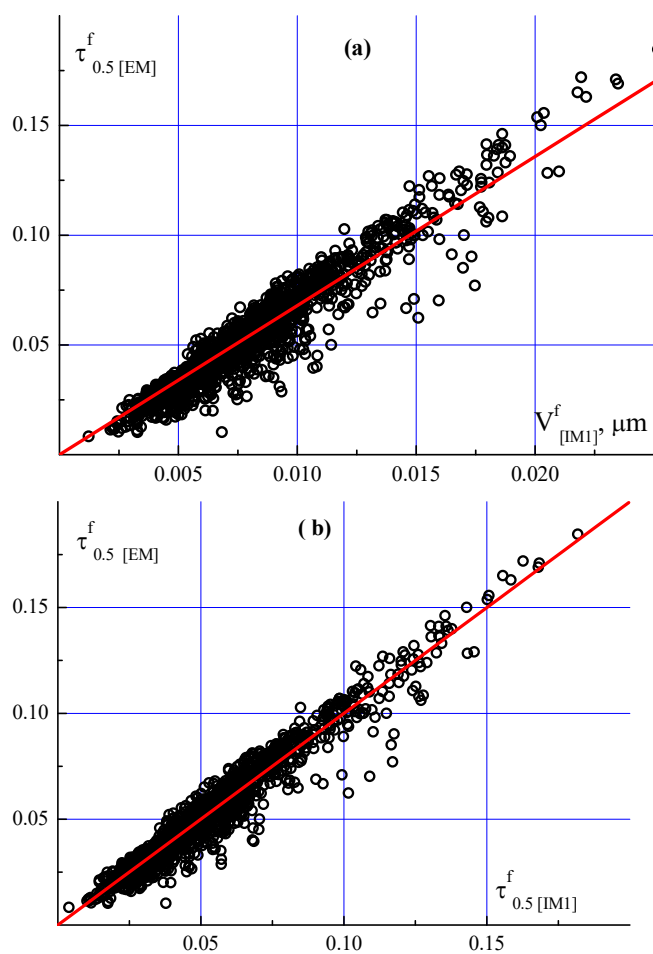
Fig. 4. (a) Interrelation between \tau_{0.5}^f and particle volume V^f and (b) interrelation between \tau_{0.5}^f values, calculated using inversion (IM1) and empirical (EM) methods
