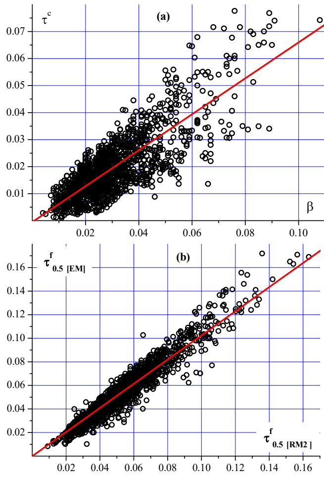
Fig. 3. (a) Interrelation of \tau^c with the parameter \beta and (b) interrelation of \tau_{0.5}^f , calculated using the base (EM) and RM2 methods
