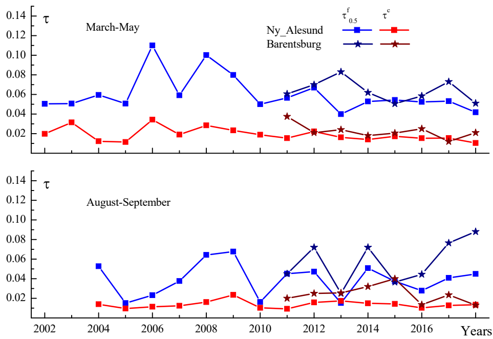
Fig. 7. Multiyear variations in \tau_{0.5}^f and \tau^c for the periods of spring maximum and fall minimum of AOD in two regions of Spitsbergen
