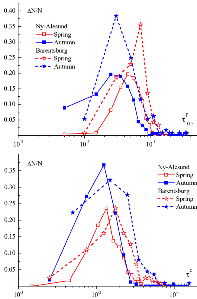
Fig. 12. Frequency histograms of (a) \tau_{0.5}^f and (b) \tau^c in spring and fall in two regions of Spitsbergen (2011-2018)
