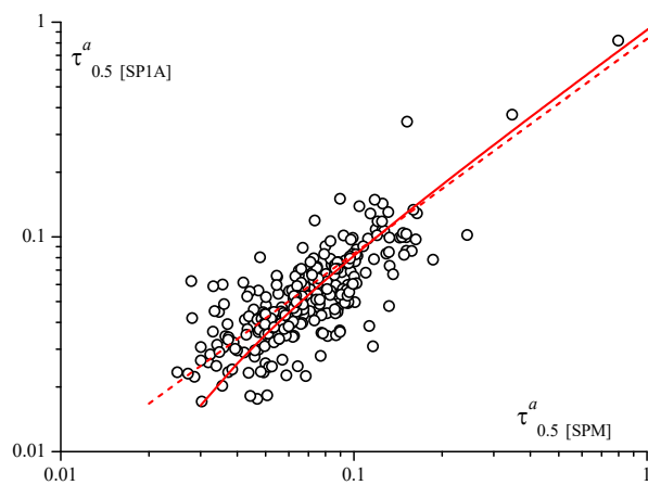
620 Fig. 9. Interrelation between Daily AOD ( 0.5 \mu\text{m} ) values, measured in Ny-Ålesund and Barentsburg (2011-2018)
