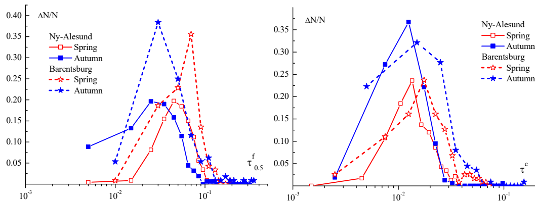
Fig. 12. Frequency histograms of (a) \tau_{0.5}^f and (b) \tau^c in spring and fall in two regions of Spitsberg (2011-2018)
