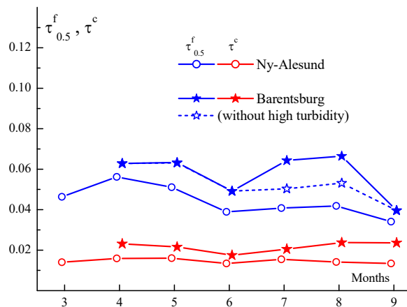
Fig. 10. Seasonal variations in fine and coarse AOD components in Ny-Ålesund and Barentsburg
