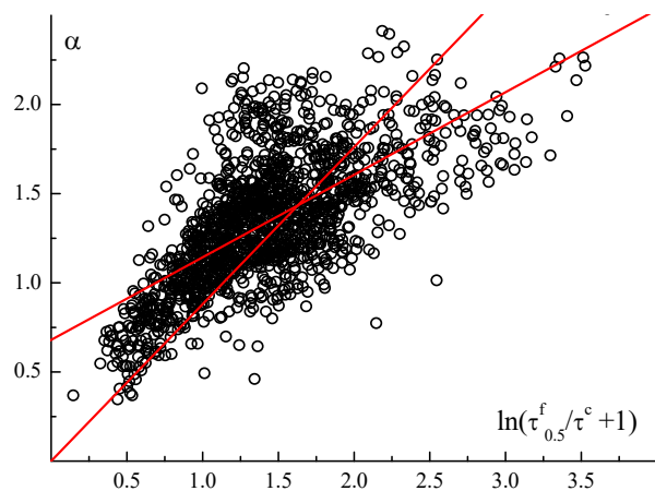
Fig. 2. Correlation dependence between the exponent \alpha and the ratio (\tau_{0.5}^f / \tau^c) according to measurements in Barentsburg
