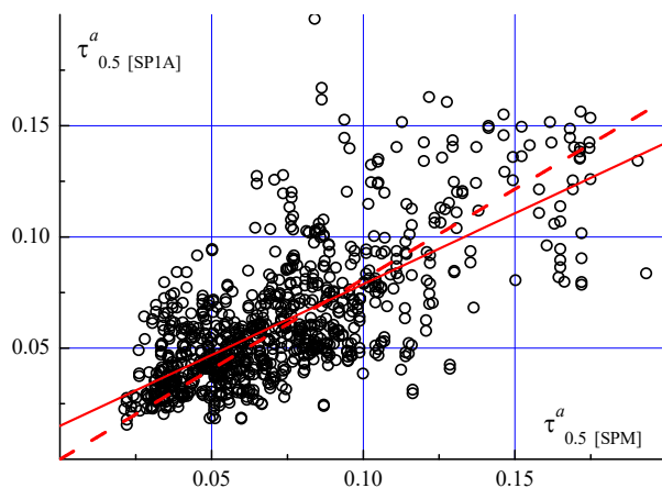
600 Fig. 1. Scatter diagram of AOD measurements in two regions using SP1A (Ny-Ålesund) and SPM (Barentsburg) photometers
