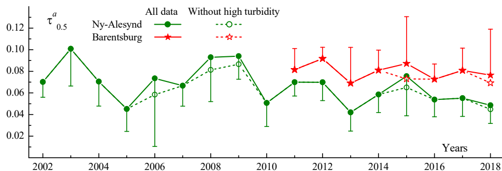
Fig. 6. Multiyear variations in Annual AOD in Ny-Ålesund and Barentsburg
