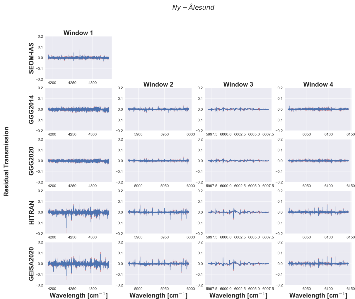
Figure 1. Example residual transmission spectra calculated from measured and fitted spectra from the Ny-Ålesund in 2019. The blue line indicates an example of the fit residual between the calculated transmission and the measured transmission. The red lines indicates the standard deviation of the residual, based on all spectra taken over the entire dataset. The columns of this figure identify the residuals of a specific window, and the rows a specific database, as identified in the axis labels.
