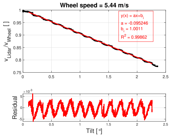
Figure 13. Example of calibration measurement made with a reference speed 5.44 m=s and a focus distance of 1.53 m. The black curve is the measurement data and the red a least-squares fit of a straight line to the data. In the lower panels is shown the residuals of the fit showing some distinct oscillations because of the speed estimation jumping from bin to bin due to the very narrow beam.
