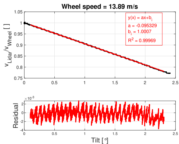
Figure 14. Example of calibration measurement made with a reference speed 13.89 m=s and a focus distance of 1.53 m.
