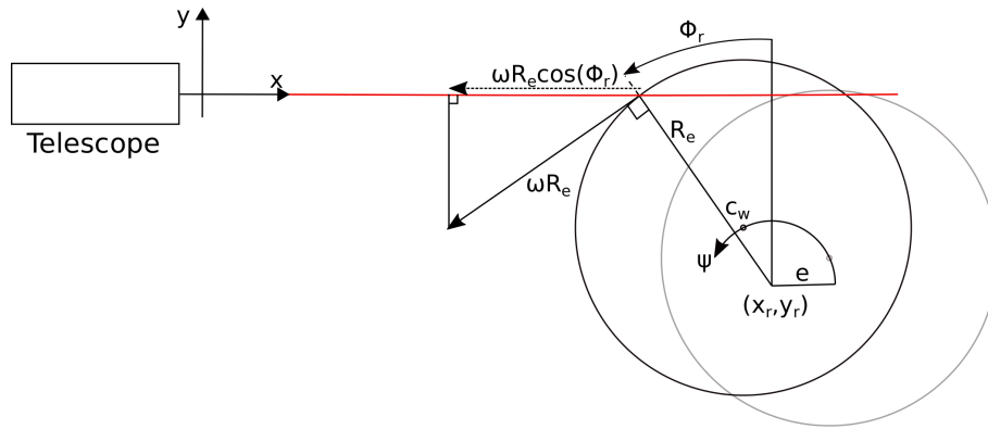
Figure 6. Schematic drawing of the influence of the wheel not rotating around its centre point. The wheel rotates around the point (x_r, y_r) which is off-sat from the wheel centre, c_w , by e .
