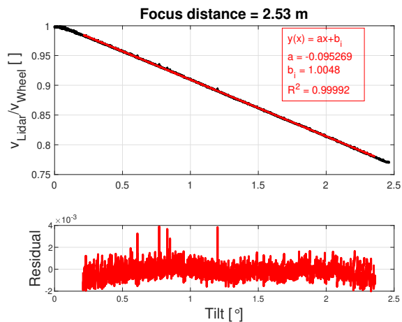
Figure 10. Example of calibration measurement made with a focus setting of 2.53 m. The black curve is the measurement data and the red a least-squares fit of a straight line to the data. In the lower panels is shown the residuals of the fit.
