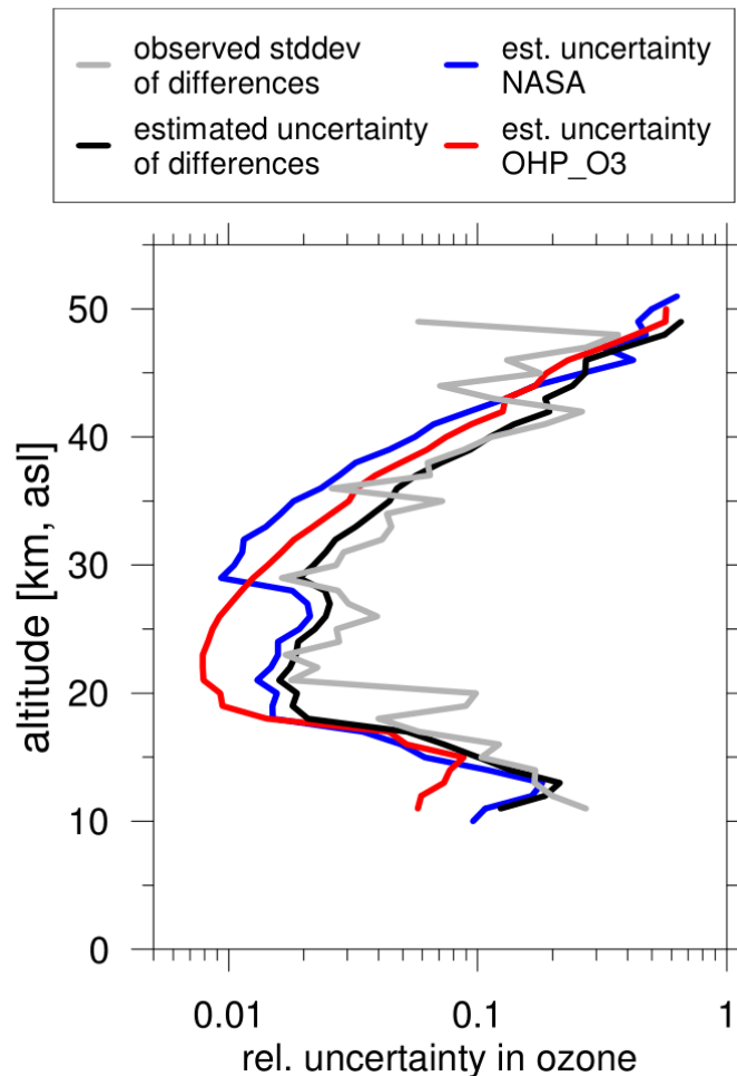
Figure 10. Vertical profiles of relative ozone uncertainties. Red: estimated by the LiO 3 S retrieval. Blue: estimated by the NASA-STROZ retrieval. Black: estimated for the relative ozone difference between NASA-STROZ and LiO 3 S ( O_3(NASA)/O_3(OHP) - 1 ). Grey: observed standard deviation for the relative ozone differences between NASA-STROZ and LiO 3 S during LAVANDE.
