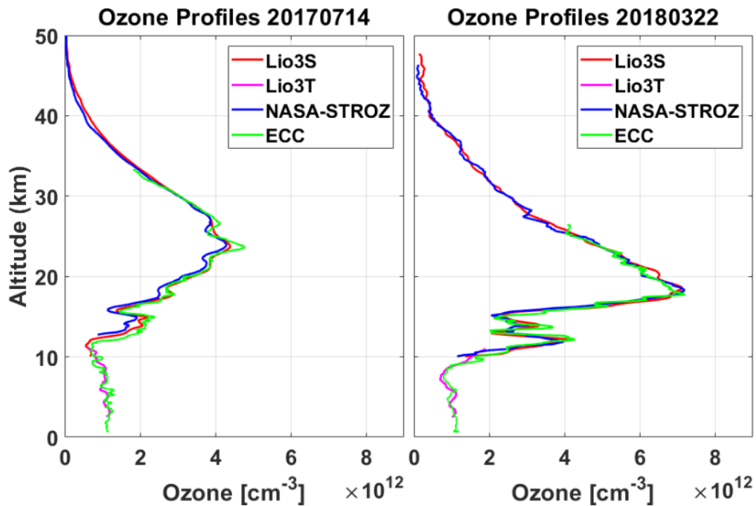
Figure 2. Ozone profiles measured by the different instruments at Observatoire de Haute-Provence on the nights July 14/15, 2017 and March 22/23, 2018. Note the seasonal differences in the character of the ozone profiles in spring and summer.
