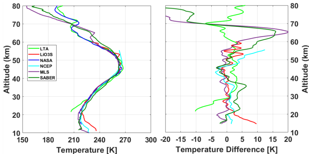
Figure 5. Satellite, NCEP, and lidar temperature profiles measured on the night of July 24/25, 2017 at or near the Observatoire de Haute-Provence (left) and temperature difference profiles with respect to the NASA temperature profile (right). All profiles have been converted to the same 300 m vertical spacing altitude grid. For MLS and SABER, the weighted average profile is calculated based on the distance in time and space between the individual satellite profiles and the OHP station.
