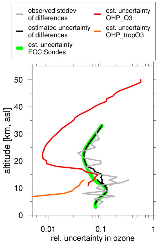
Figure 11. Vertical profiles of estimated relative ozone uncertainties for ECC sonde ozone profiles (green line, two times the estimate from Tarasick et al. (2016), excluding radiosonde pressure errors) and ozone measurement uncertainty estimated by the LiO 3 S retrieval (red line), and the LiO 3 T (orange line). Black: estimated combined uncertainty for the relative ozone difference between ECC sondes and the two LiO 3 S (tropospheric system up to 13 km, stratospheric system above 10 km). Grey: corresponding observed standard deviation for the relative ozone differences during LAVANDE.
