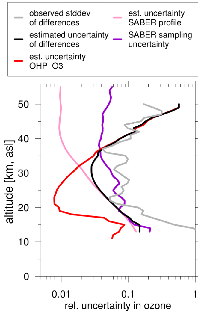
Figure 13. Vertical profiles of estimated relative ozone measurement uncertainties for individual SABER profiles (pink line, from Rong et al., 2009), SABER spatial variation / sampling uncertainty over the colocation box (purple line), and LiO 3 S measurement uncertainty (red line). Estimated combined uncertainty for the relative ozone difference SABER minus LiO 3 S based on SABER individual profile uncertainty is given by the black line. The grey line gives observed standard deviation of the relative ozone differences between SABER and LiO 3 S.
