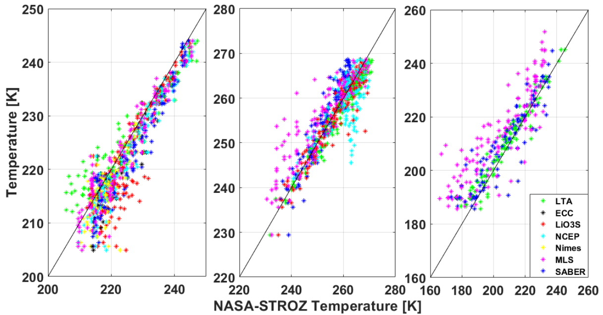
Figure 16. Scatter plots of temperature as measured by the various LAVANDE instruments (along the vertical axis) and temperature measured by NASA-STROZ (along the horizontal axis). Left: Temperature from 12 to 35 km altitude. Centre: Temperature from 35 to 60 km altitude. Right: Temperature from 60 to 80 km altitude.
