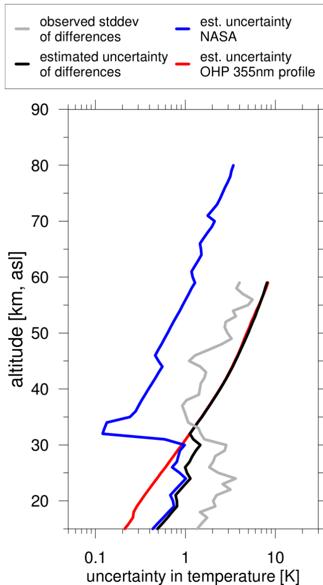
Figure 18. Similar to Figs. 10 to 13, but for temperature. Plotted are: estimated measurement uncertainty for temperature measured by LiO 3 S (red curve) and NASA-STROZ (blue curve), estimated combined uncertainty for temperature differences between the two systems (black curve), and observed standard deviation of temperature differences between the two systems (grey curve) during LAVANDE.
