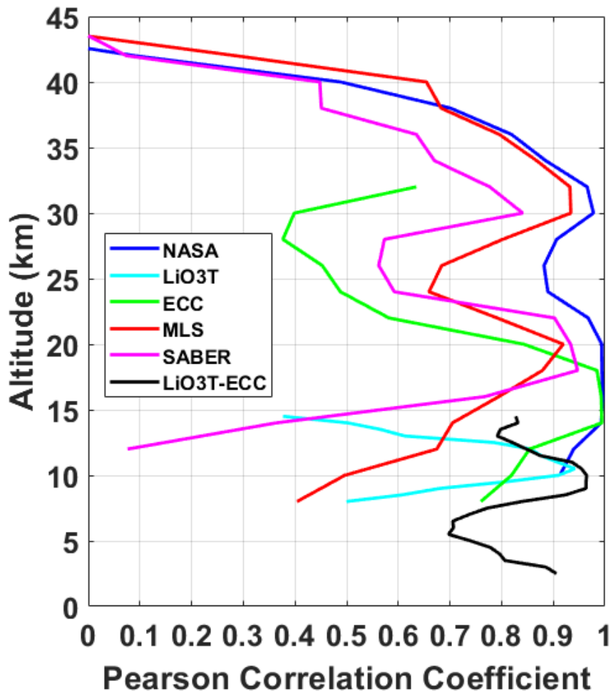
Figure 9. Vertical profiles of the correlation of ozone concentrations measured by the various LAVANDE instruments and ozone concentration measured by the LiO 3 S (outliers were excluded). Correlation is taken over the 28 nights of the LAVANDE campaign and over 2 kilometres in altitude. Results for MLS and SABER are calculated from the weighted average profiles. Slightly smaller correlations were obtained for the closest match SABER or MLS profiles (not shown).
