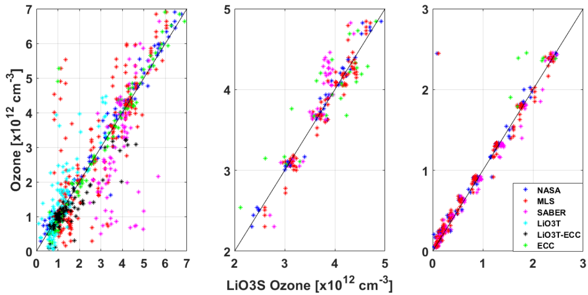
Figure 8. Scatter plots of ozone concentration as measured by the various LAVANDE instruments (along the vertical axis) and ozone measured by the LiO 3 S (along the horizontal axis). Left: Ozone from 0 to 20 km altitude. Centre: Ozone from 20 to 30 km altitude. Right: Ozone from 30 to 50 km altitude.
