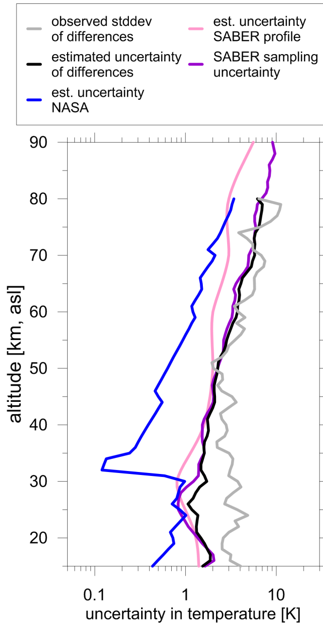
Figure 21. Same as Fig. 20, but for SABER satellite temperature profiles (pink for measurement uncertainty and purple for sampling uncertainty) and NASA-STROZ (blue for measurement uncertainty). Results for SABER are shown for the weighted average profiles, but very similar results are obtained for closest match SABER profiles. SABER single profile temperature measurement uncertainty was estimated following Rezac et al. (2015a, b).
