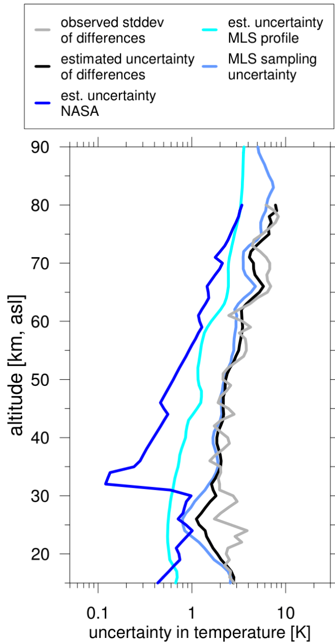
Figure 20. Same as Figs. 18 and 19, but comparing measurement and sampling uncertainties of MLS satellite temperature profiles (cyan and light blue curves) and NASA-STROZ ground-based profiles (dark blue). Results are for the MLS weighted average profiles, but very similar results are obtained for closest match MLS profiles. MLS single profile measurement uncertainty is included in the data distribution and is described in Schwartz et al. (2008)
