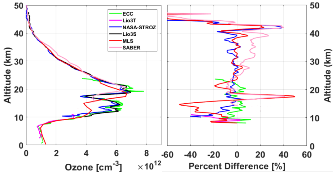
Figure 4. Satellite and lidar ozone profiles measured on the night March 19/20, 2018 at or near the Observatoire de Haute-Provence (left). Percent differences for each profile with respect to the LiO 3 S profile (right). All profiles have been converted to the same 300 m vertical spacing altitude grid. For MLS and SABER, the weighted average profile is calculated based on the distance in time and space between the individual satellite profiles and the OHP station.
