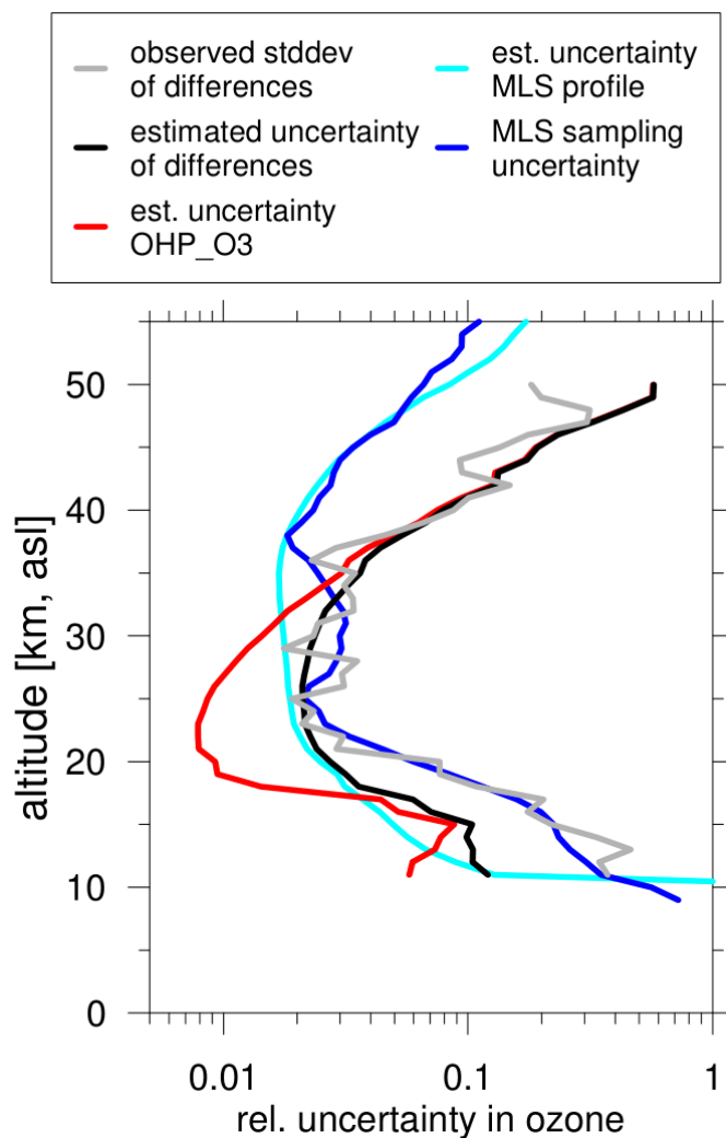
Figure 12. Vertical profiles of estimated relative ozone uncertainties for individual MLS profiles (Froidevaux et al., 2008) from the MLS data files (cyan line), and MLS spatial variation / sampling uncertainty estimated from all profiles in the collocation box (blue line). LiO 3 S ozone uncertainty (red line). Estimated uncertainty for the relative ozone difference (MLS minus LiO 3 S) based on MLS individual profile uncertainty is given by the black line. The grey line gives the observed standard deviation of the relative ozone differences between MLS and LiO 3 S during LAVANDE.
