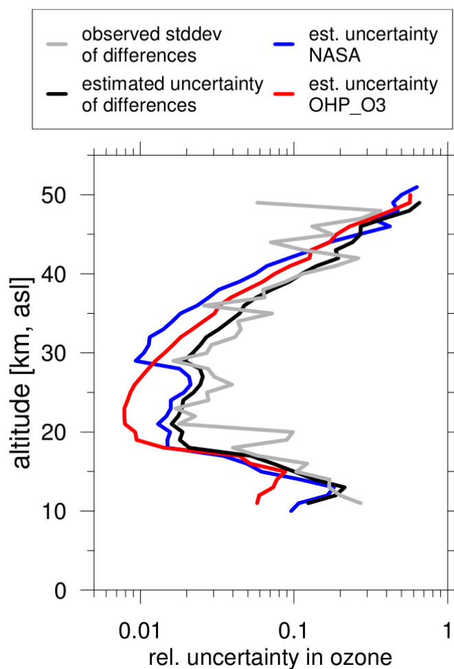
Figure 10. Vertical profiles of relative ozone uncertainties. Red: estimated by the \text{LiO}_3\text{S} retrieval. Blue: estimated by the NASA-STROZ retrieval. Black: estimated for the relative ozone difference between NASA-STROZ and \text{LiO}_3\text{S} ( O_3(\text{NASA})/O_3(\text{OHP}) - 1 ). Grey: observed standard deviation for the relative ozone differences between NASA-STROZ and \text{LiO}_3\text{S} during LAVANDE.
