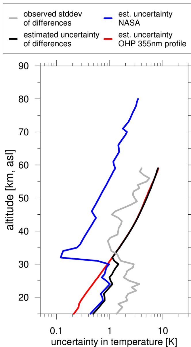
Figure 18. Similar to Figs. 10 to 13, but for temperature. Plotted are: estimated uncertainty for temperature measured by LiO 3 S (red curve) and NASA-STROZ (blue curve), estimated uncertainty for temperature differences between the two systems (black curve), and observed standard deviation of temperature differences between the two systems (grey curve) during LAVANDE.
