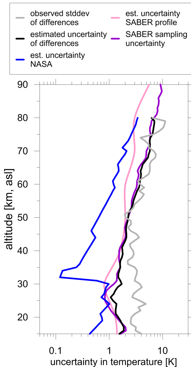
Figure 21. Same as Fig. 20, but for SABER satellite temperature profiles (pink and purple curves) and NASA-STROZ. Results for SABER are shown for the weighted average profiles, but very similar results are obtained for closest match SABER profiles. SABER single profile temperature uncertainty was estimated following Rezac et al. (2015a, b).
