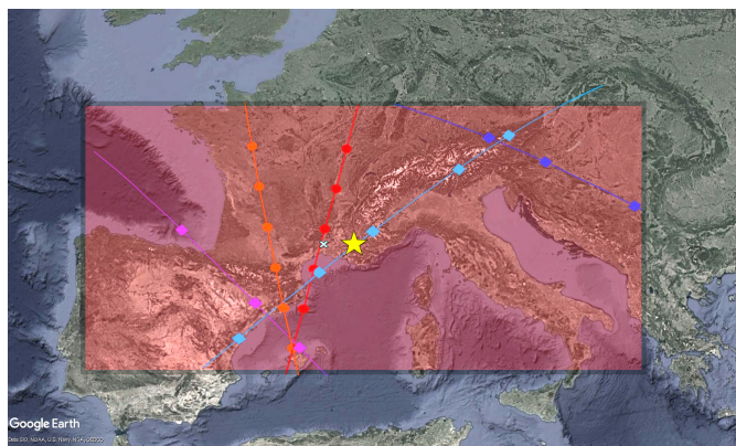
Figure 1. The area defined for coincident measurements during the LAVANDE campaign (39,-9) to (49,21). L'Observatoire de Haute-Provence is represented by the yellow star at (43.93,5.71) and Nîmes radiosonde launches by a cyan X at (43.86,4.41). Ascending (red) and descending (orange) orbits for MLS with tangent point locations of profiles for 17 July 2018. Ascending (light blue) and descending (purple and dark blue) orbits for SABER with tangent point locations of profiles for 17 July 2018. (data: © Google Earth Pro, 2019)
