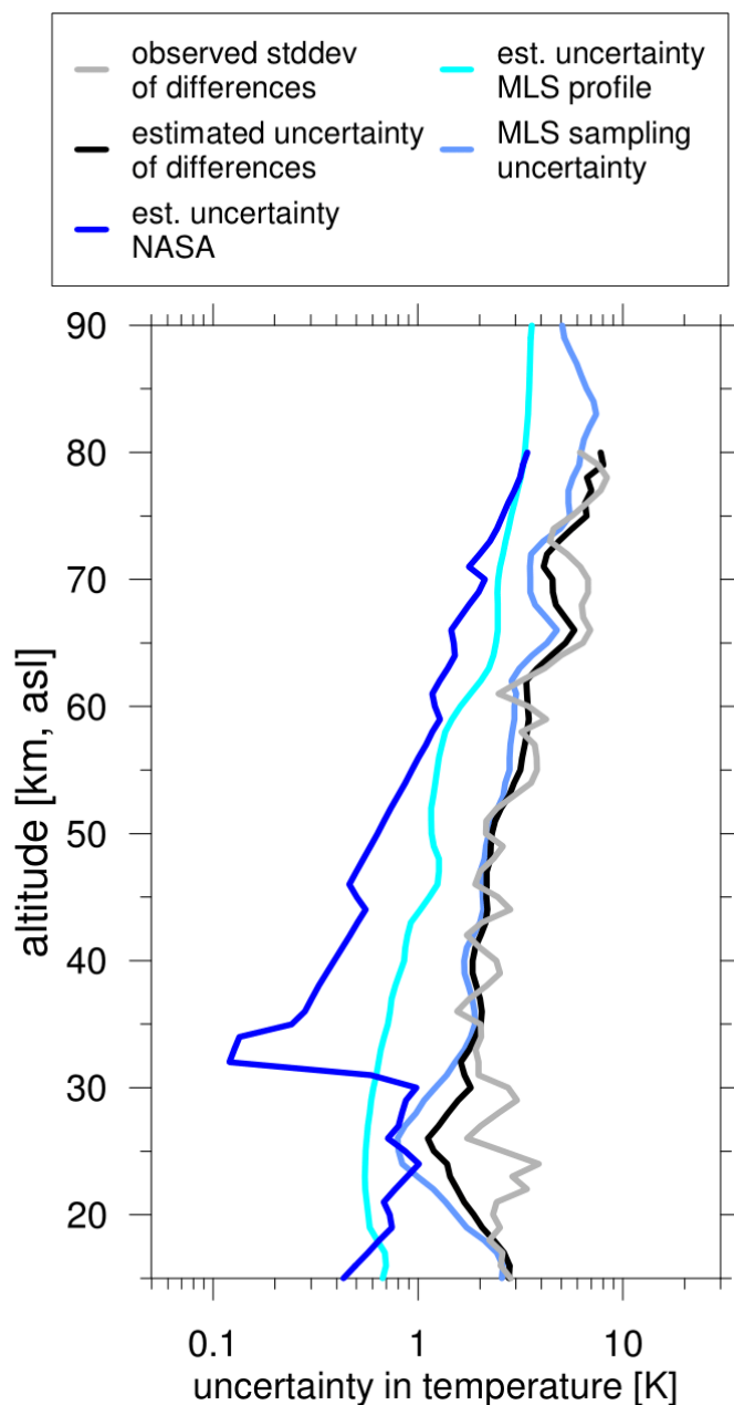
Figure 20. Same as Figs. 18 and 19, but comparing single profile and sampling uncertainties of MLS satellite temperature profiles (cyan and light blue curves) and NASA-STROZ ground-based profiles. Results are for the MLS weighted average profiles, but very similar results are obtained for closest match MLS profiles. MLS single profile uncertainty is included in the data distribution and is described in Schwartz et al. (2008)
