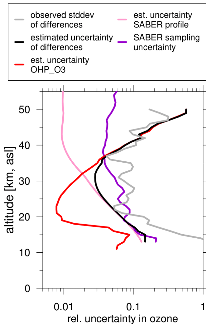
Figure 13. Vertical profiles of estimated relative ozone uncertainties for individual SABER profiles (pink line, from Rong et al., 2009), SABER spatial variation / sampling uncertainty over the collocation box (purple line), and LiO 3 S ozone uncertainty (red line). Estimated uncertainty for the relative ozone difference SABER minus LiO 3 S based on SABER individual profile uncertainty is given by the black line. The grey line gives observed standard deviation of the relative ozone differences between SABER and LiO 3 S.
