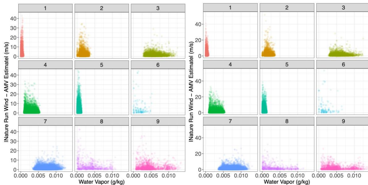
603 Figure 7: Scatterplot of Water Vapor vs Absolute Tracked Wind Error, each sub-panel corresponding to the 604 specific Gaussian mixture component to which each point in the testing set has been assigned. (A): U- 605 Direction Wind (B): V-Direction Wind.
