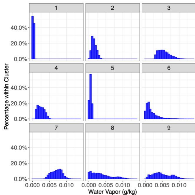
606 Figure 8: Histogram of Nature Run water vapor for each cluster identified by the Gaussian mixture model, 607 applied to the testing set. Each sub-panel represents the cluster each point was assigned to. 608
