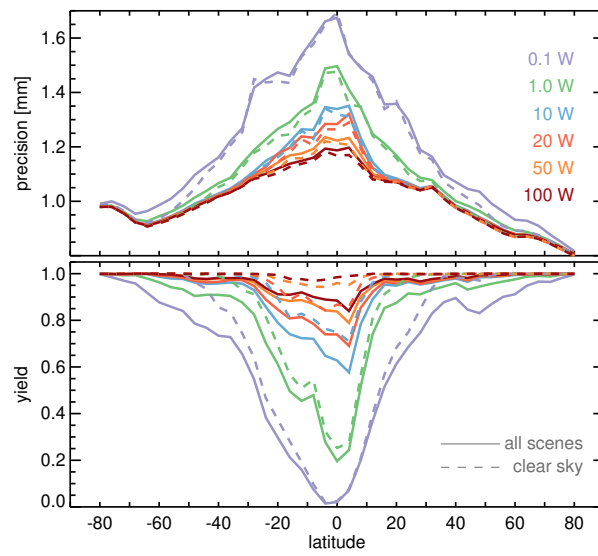
Figure 7. Total column water vapor precision (top) as well as fractional yield (bottom) for different transmit powers versus latitude.
