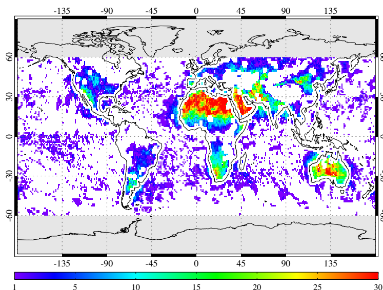
Figure 3. Location and frequency of the 1^\circ \times 1^\circ cloud-free latitude/longitude boxes that were selected by the algorithm every two weeks for the period from May 2018 until February 2020.
